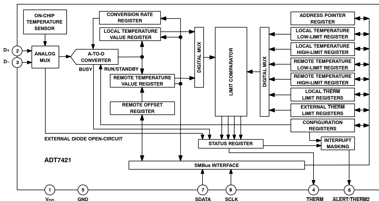
Figure 1. Block Diagram
