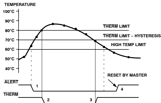
Figure 14. Operation of the \overline{\text{ALERT}} and \overline{\text{THERM}} Interrupts
