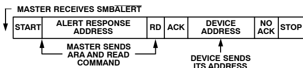
Figure 13. Use of \text{SMBALERT}
