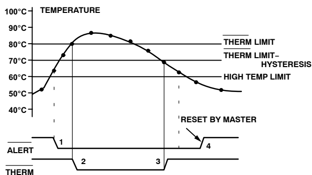
Figure 14. Operation of the \overline{\text{ALERT}} and \overline{\text{THERM}} Interrupts
