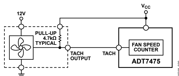
Figure 36. Fan with TACH Pull-Up to V CC
