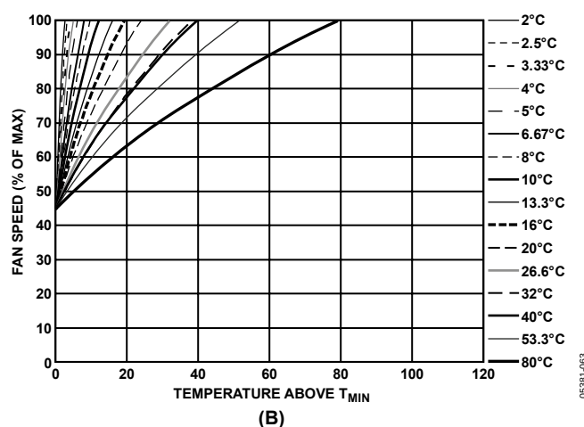
Figure 58. T_{\text{RANGE}} and % Fan Speed Slopes with \text{PWM}_{\text{MIN}} = 20\%
