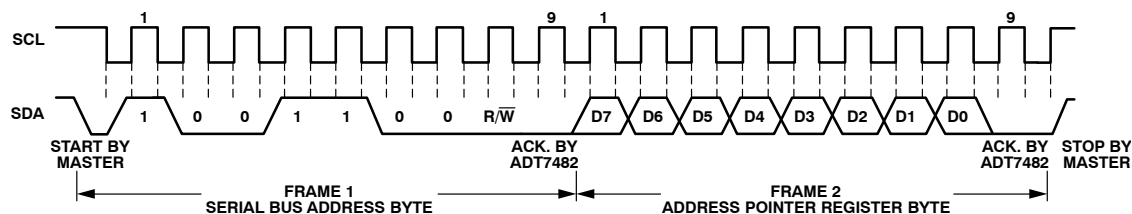
Figure 17. Writing to the Address Pointer Register Only
