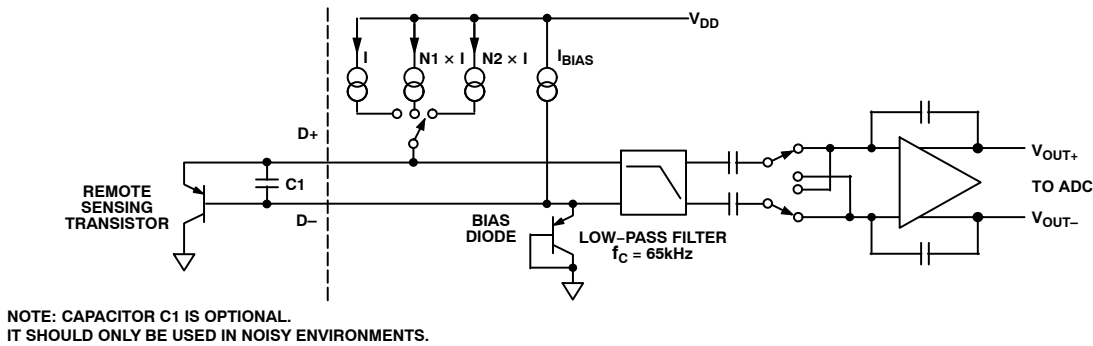
Figure 15. Input Signal Conditioning
