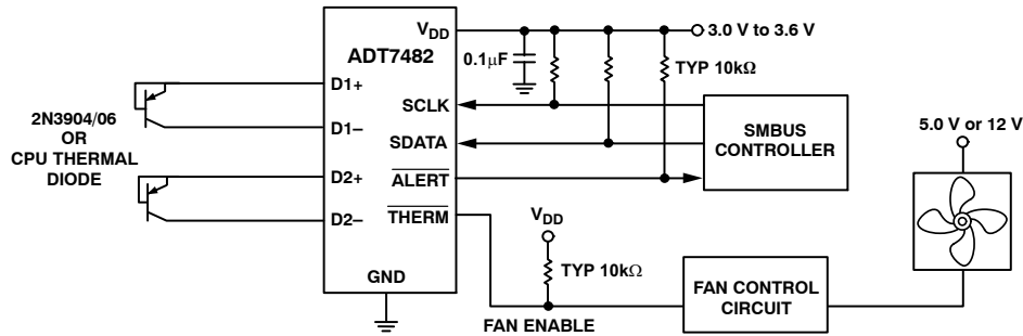
Figure 24. Typical Application Circuit
