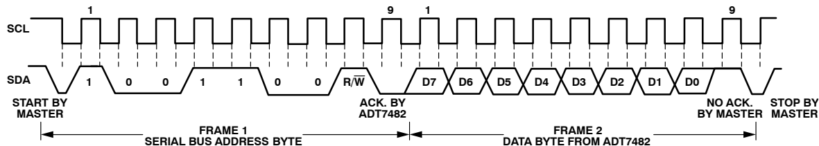
Figure 18. Reading from a Previously Selected Register
