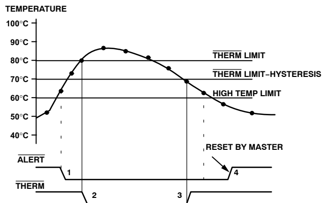
Figure 20. Operation of the \overline{\text{ALERT}} and \overline{\text{THERM}} Interrupts
