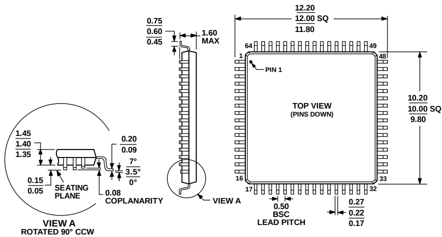
COMPLIANT TO JEDEC STANDARDS MS-026-BCD Figure 99. 64-Lead Low Profile Quad Flat Package [LQFP] (ST-64-2) Dimensions shown in millimeters
