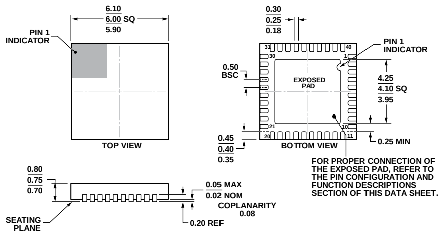
Figure 97. 40-Lead Lead Frame Chip Scale Package [LFCSP_WQ] 6 × 6 mm Body, Very Very Thin Quad (CP-40-9) Dimensions shown in millimeters
