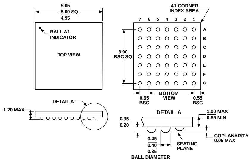
Figure 102. 49-Ball Chip Scale Package Ball Grid Array [CSP_BGA] (BC-49-1)
