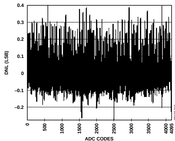
Figure 11. Typical DNL Error, Temperature 25°C, V_{REF} = Internal 2.5 V, Single-Ended Mode ADCCP = DAC1/ADC13, ADCCN = ADC0, Sampling Rate = 345 kHz Worst Case Positive = 0.40 LSB, Code 607 Worst Case Negative = -0.27 LSB, Code 2486
