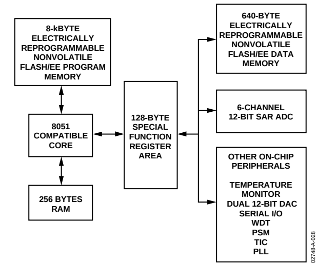
Figure 21. Programming Model
