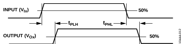
Figure 12. Propagation Delay Parameters
