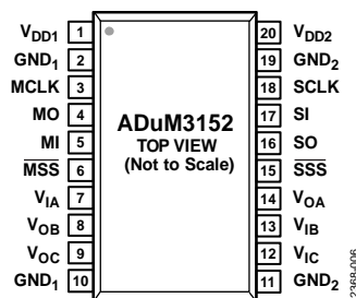
Figure 6. ADuM3152 Pin Configuration
