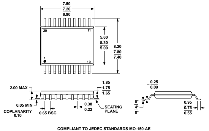
Figure 20. 20-Lead Shrink Small Outline Package [SSOP] (RS-20)
