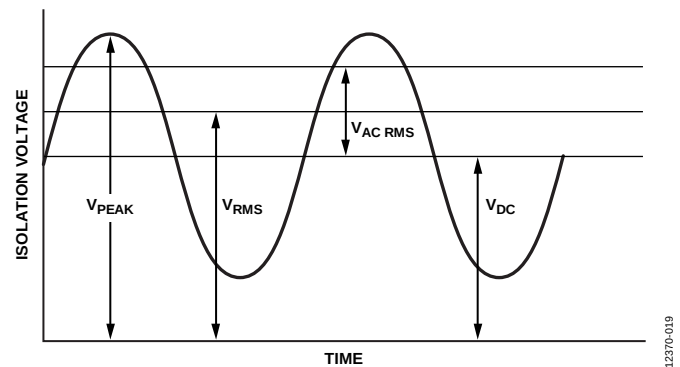
Figure 19. Critical Voltage Example
