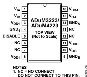
Figure 4. Pin Configuration
