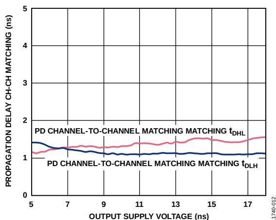
Figure 12. Typical Propagation Delay, Channel-to-Channel Matching vs. Output Supply Voltage
