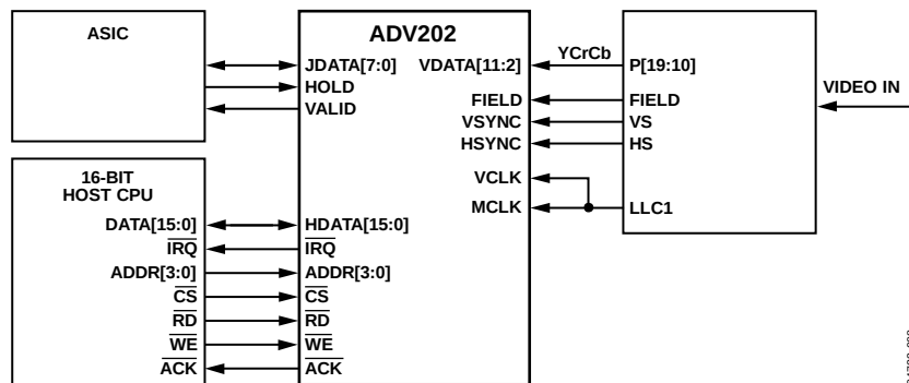
Figure 30. JDATA Application
