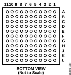
Figure 30. 121-Ball Pin Configuration
