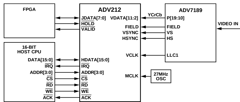
Figure 39. JDATA Application
