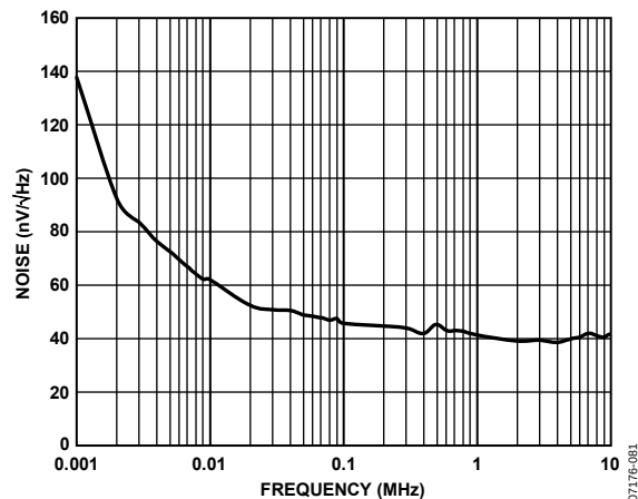
Figure 65. ADV3201 Output Noise
