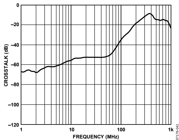
Figure 67. ADV3201 Crosstalk, One Adjacent Channel, RTO
