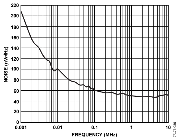
Figure 66. ADV3201 OSD Output Noise
