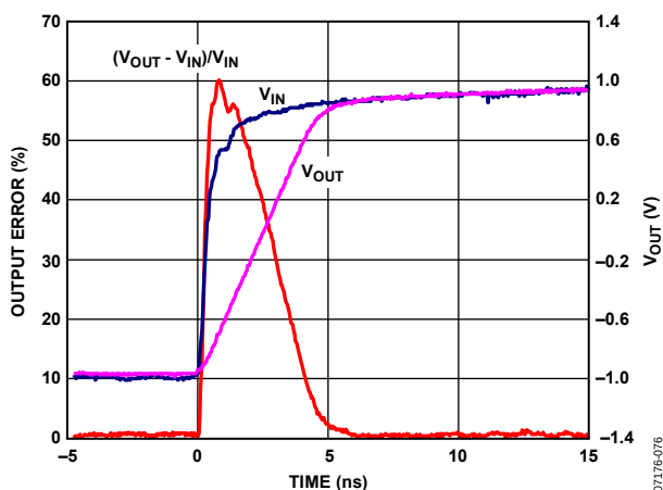
Figure 88. ADV3201 Settling Time
