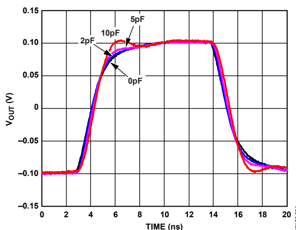
Figure 91. ADV3201 OSD Small Signal Pulse with Capacitive Loads, 200 mV p-p
