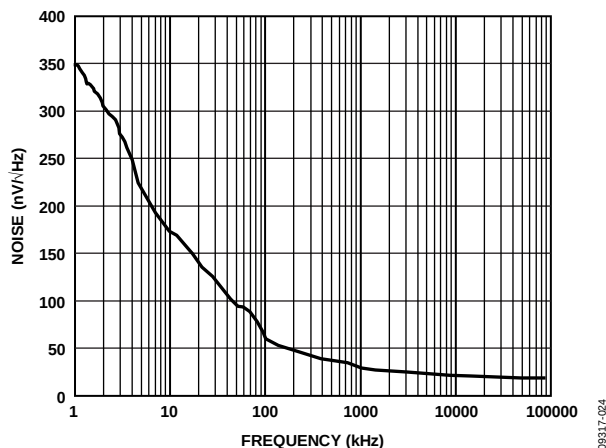
Figure 26. ADV3224 Output Noise Density, 100 Ω Load
