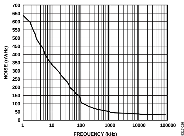
Figure 29. ADV3225 Output Noise Density, 100 Ω Load
