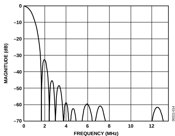
Figure 14. 0.65 MHz Low-Pass Chroma Filter
