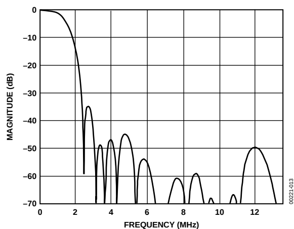
Figure 13. 1.3 MHz Low-Pass Chroma Filter
