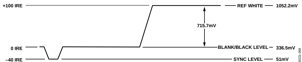
Figure 68. NTSC RGB Video Levels
