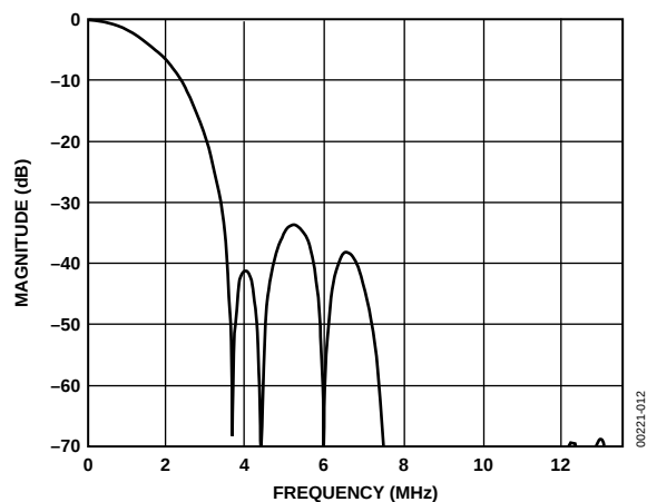
Figure 12. QCIF Luma Filter
