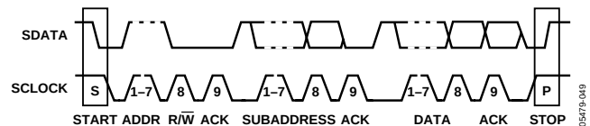
Figure 44. Bus Data Transfer
