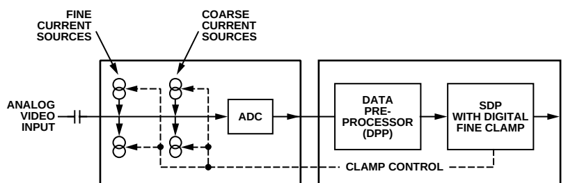
Figure 14. Clamping Overview
