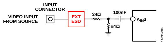
Figure 11. Single-Ended Input Network
