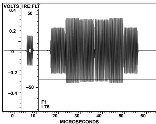
Figure 133. NTSC Luma
