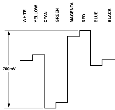
Figure 122. Pr Levels—PAL
