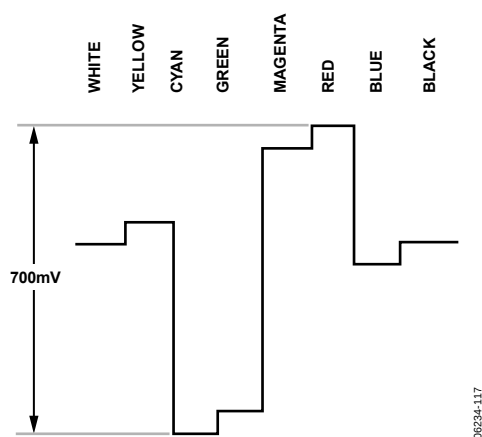
Figure 119. Pr Levels—NTSC
