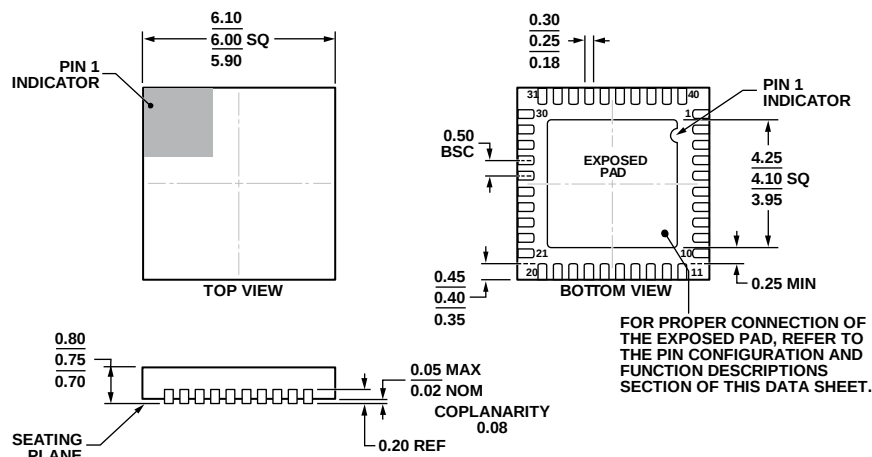
Figure 147. 40-Lead Lead Frame Chip Scale Package [LFCSP_WQ] 6 mm × 6 mm Body, Very Very Thin Quad (CP-40-9) Dimensions shown in millimeters
