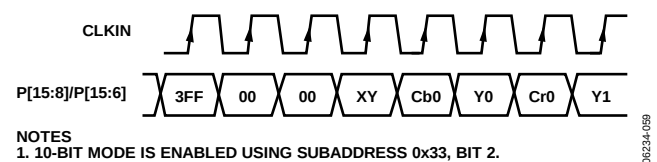
Figure 61. ED (at 54 MHz) Input Sequence (EAV/SAV)
