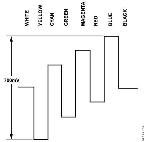
Figure 123. Pb Levels—PAL
