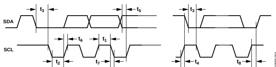
Figure 4. I 2 C Timing
