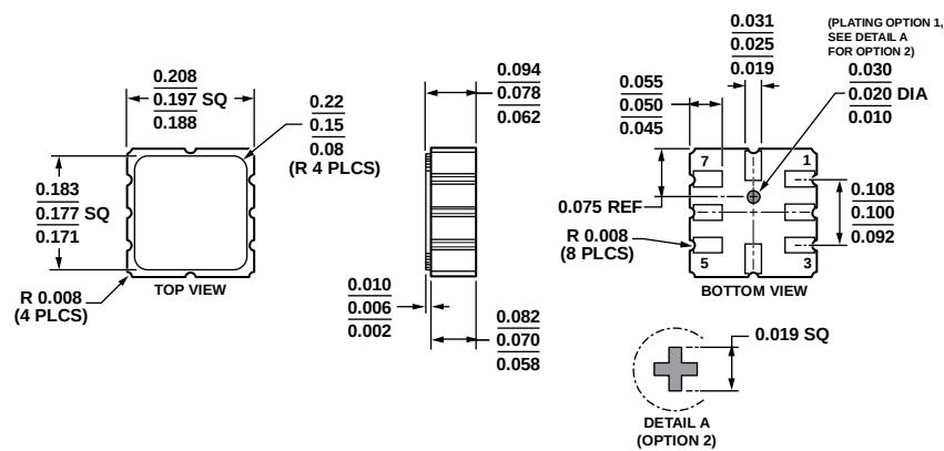
Figure 23. 8-Terminal Ceramic Leadless Chip Carrier [LCC] (E-8-1)
