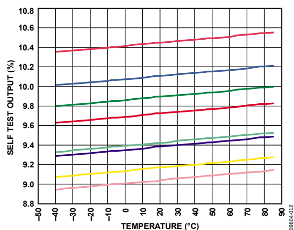
Figure 12. Self Test Response vs. Temperature
