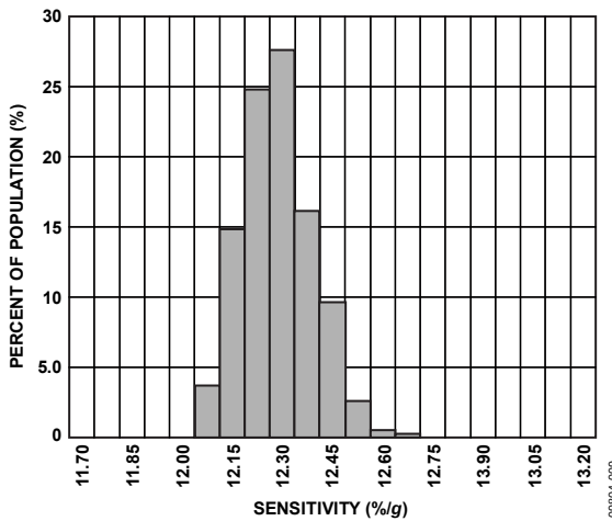
Figure 9. Y-Axis Sensitivity at 25°C
