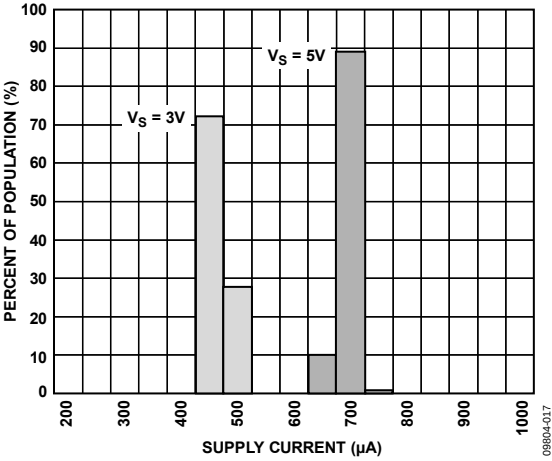
Figure 17. Supply Current at 25°C
