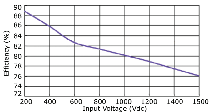
AE15-UW-S24 Efficiency Curve Efficiency vs. Input Voltage
