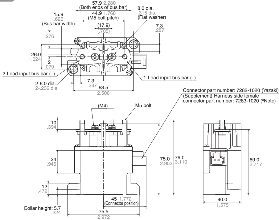
Mounting dimensions
