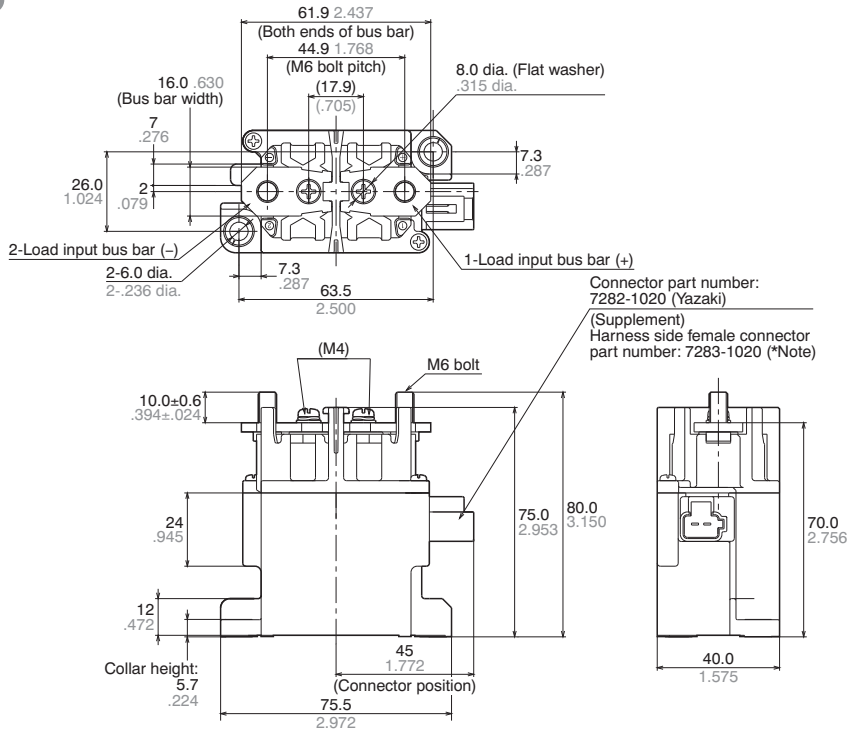
Mounting dimensions
