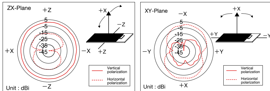
Typical characteristics of radiation pattern (@2.45GHz)
