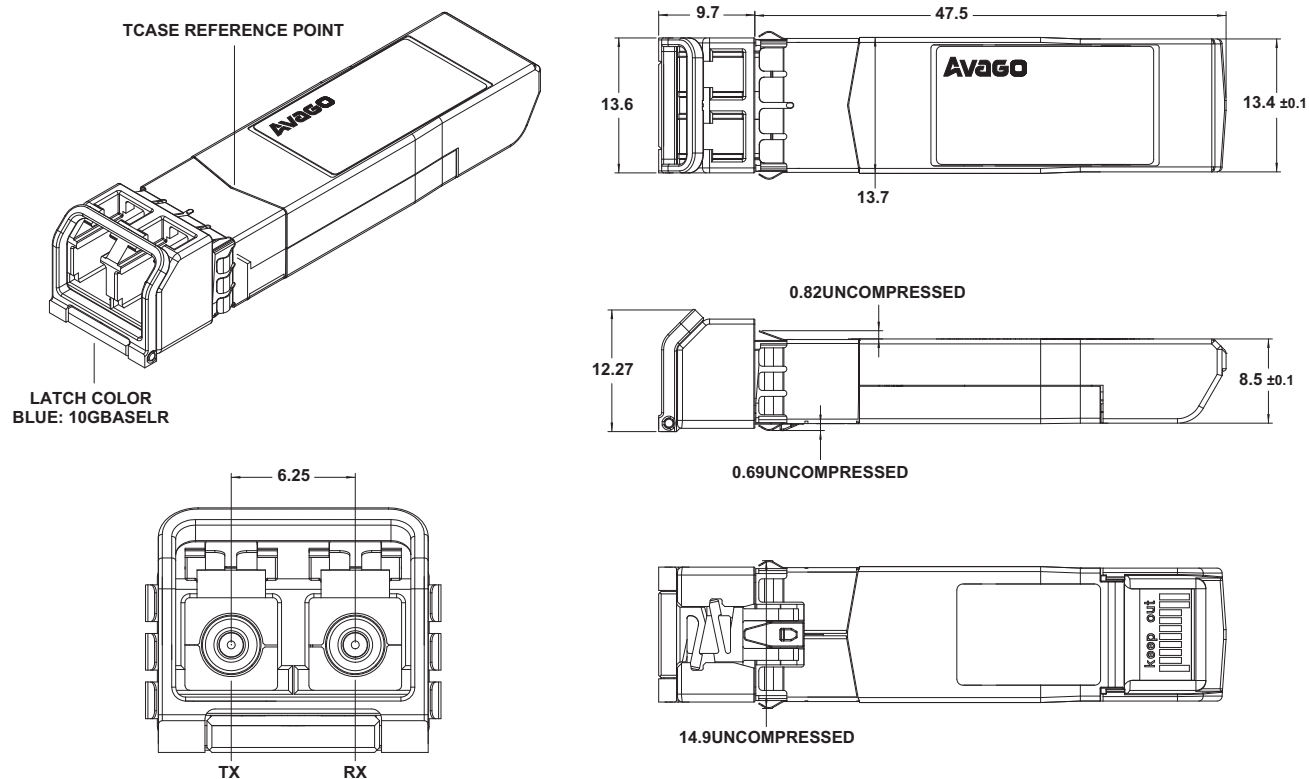
Figure 6. Module drawing
