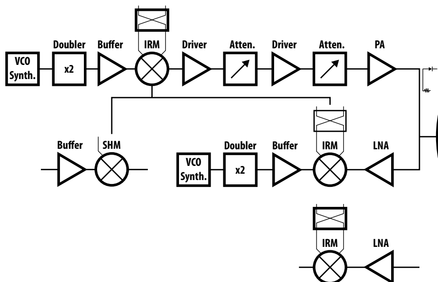
Microwave Link Packaged Suggested Solution 23 GHz
