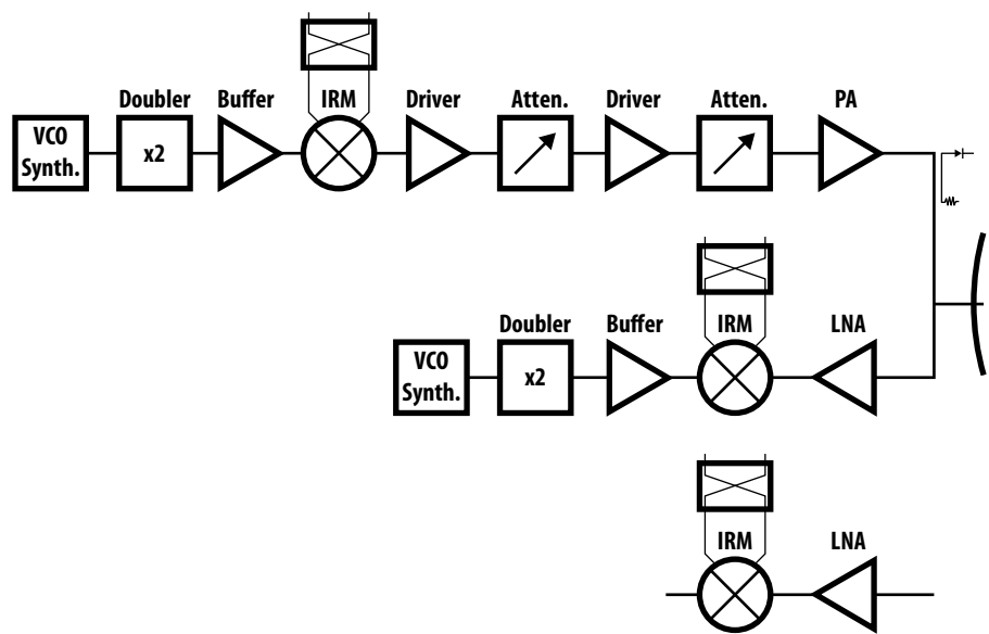
Microwave Link Packaged Suggested Solution 28 GHz
