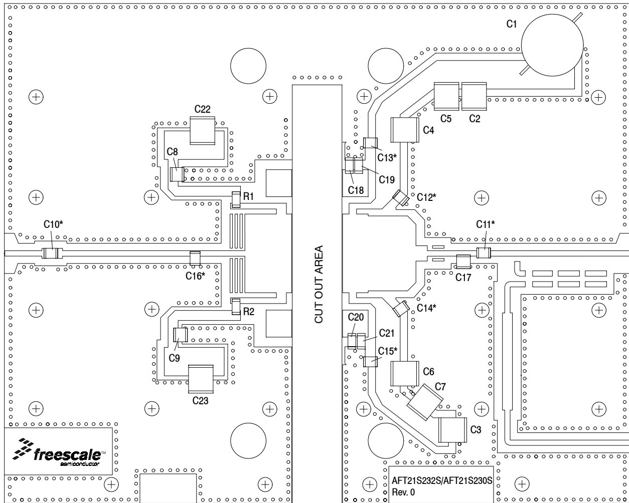
Figure 4. AFT21S230SR3(232SR3) Test Circuit Component Layout
