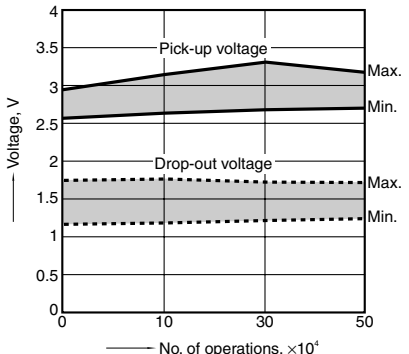
3. Mechanical life
