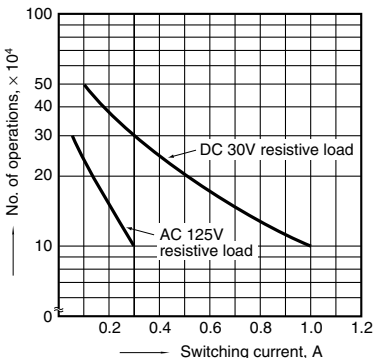
2. Life curve
