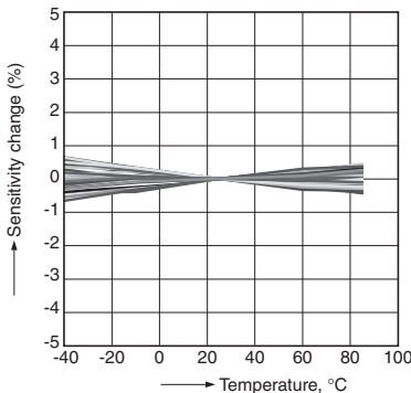
3. Sensitivity temperature characteristics (VDD=5V)
