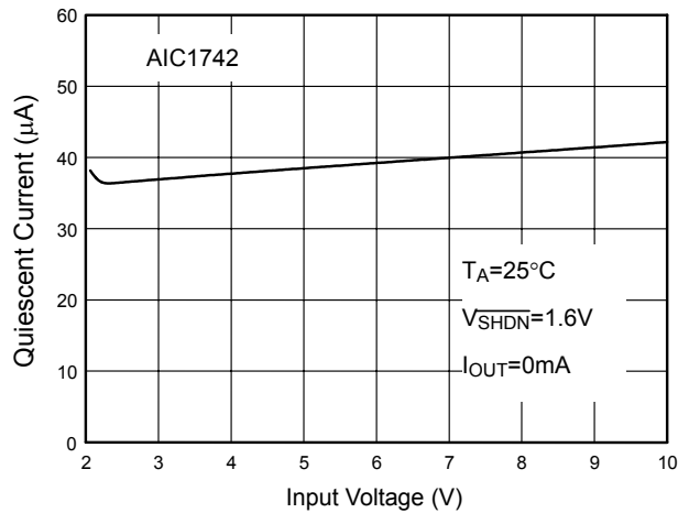
Fig. 1 Quiescent Current
