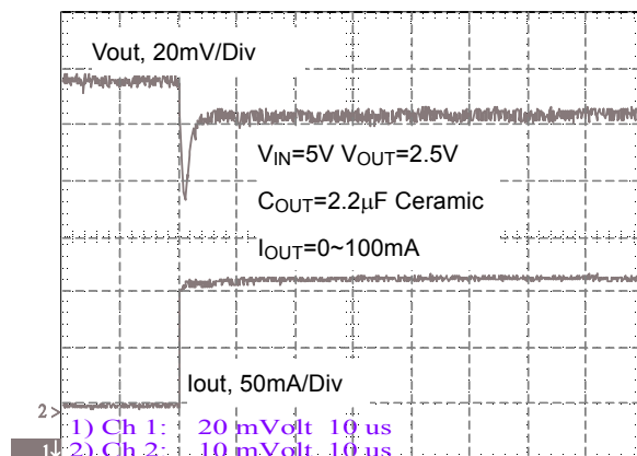
Fig. 17 Transient Response 2
