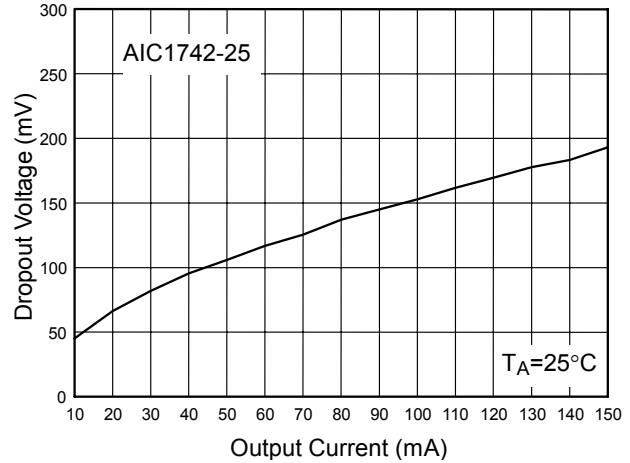
Fig. 8 Dropout Voltage
