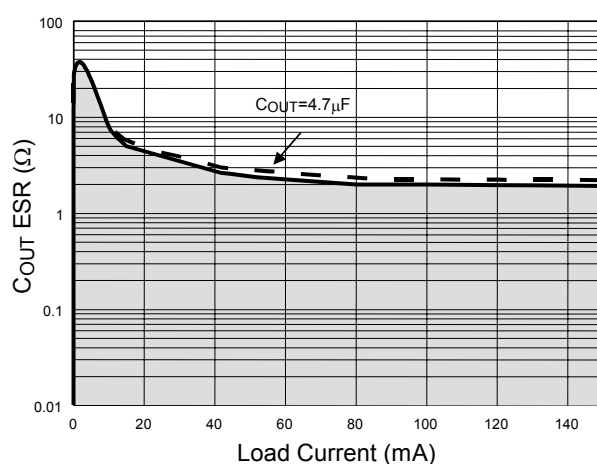
Fig. 21 Region of Stable C_{OUT} ESR vs. Load Current
