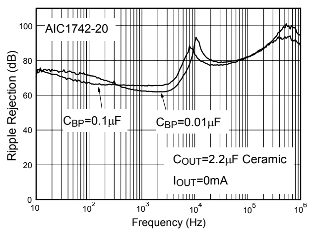
Fig. 10 Input Ripple Rejection
