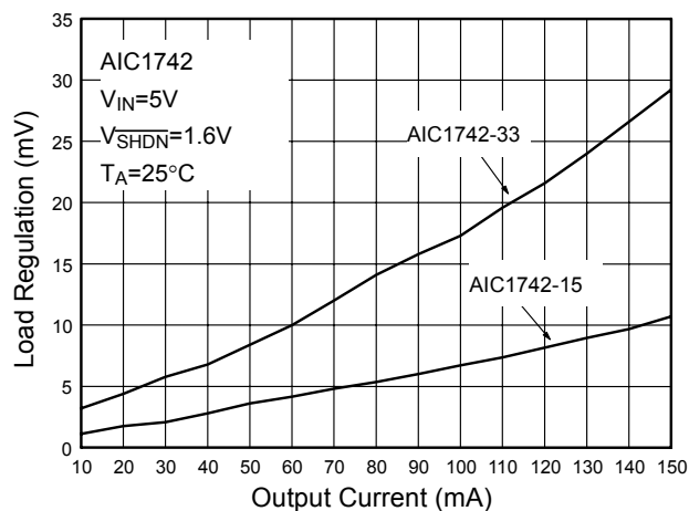
Fig. 5 Load Regulation
