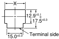
PC board pattern
