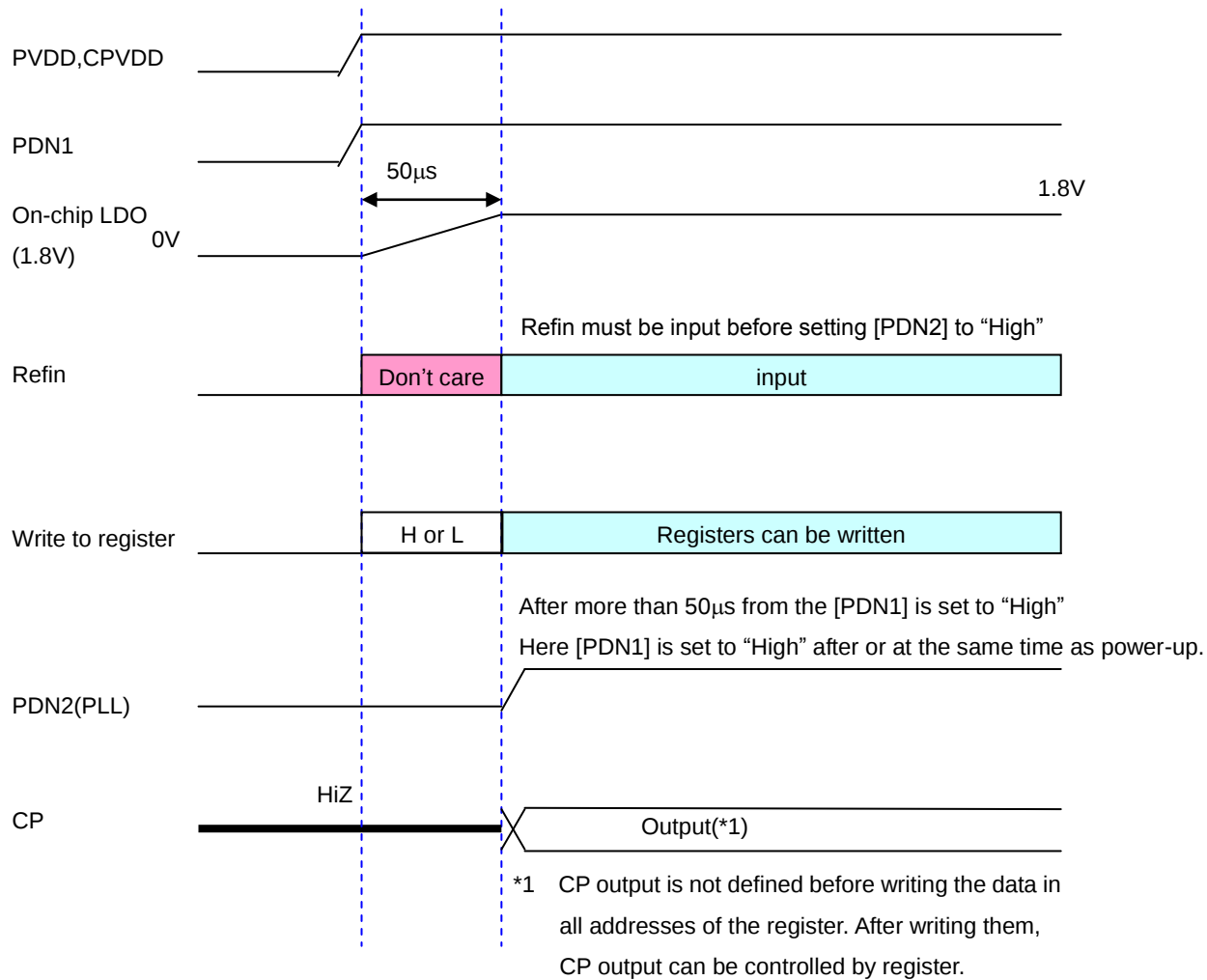
Fig. 13 Power Sequence
