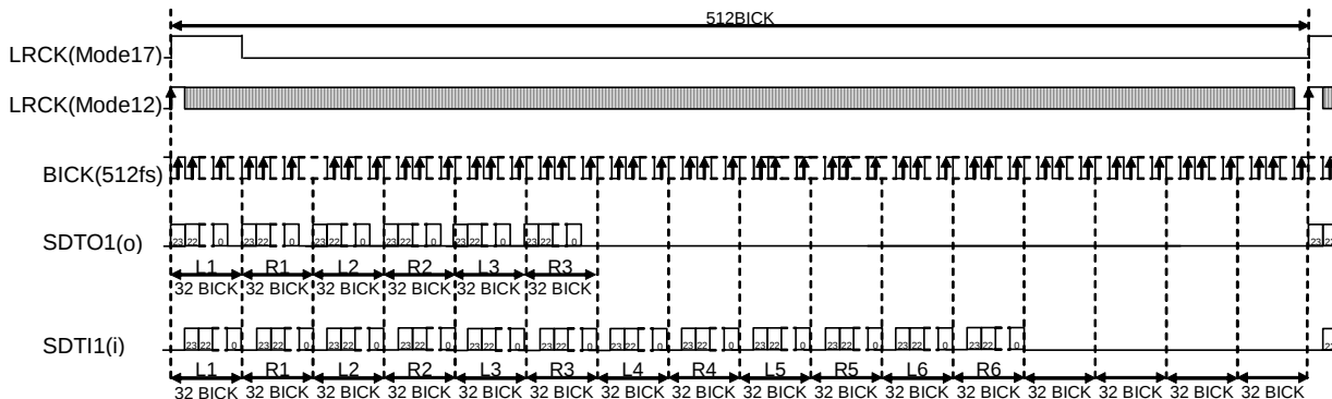
Figure 30. Mode 12/17 Timing (TDM512 Mode)
