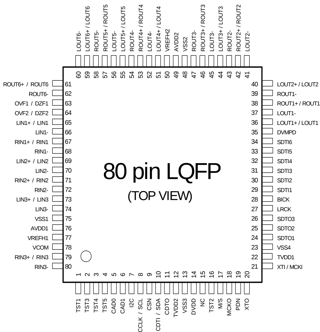
Figure 2. Pin Layout
