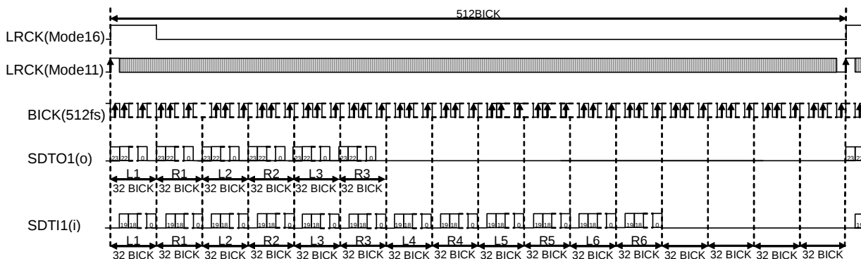
Figure 29. Mode 11/16 Timing (TDM512 Mode)
