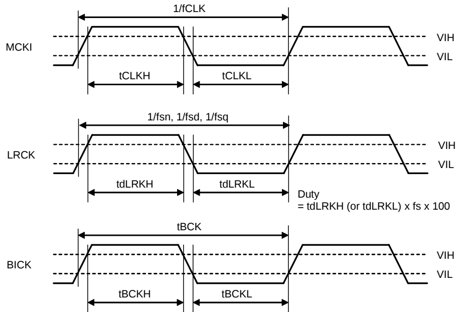
Figure 3. Clock Timing (TDM1/0 bit = "00" & Slave mode)
