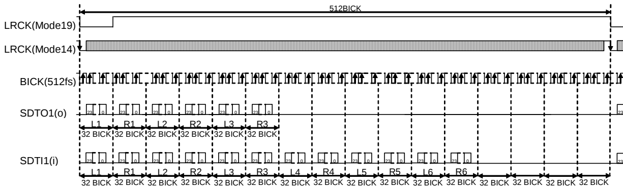
Figure 32. Mode 14/19 Timing (TDM512 Mode)
