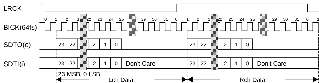
Figure 27. Mode 4/9 Timing (Stereo Mode)
