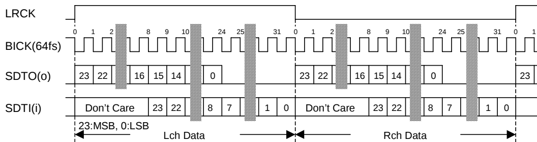
Figure 25. Mode 2/7 Timing (Stereo Mode)
