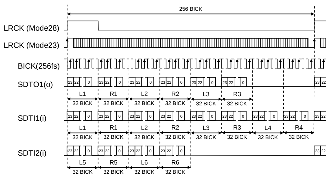
Figure 36. Mode 23/28 Timing (TDM256 Mode)
