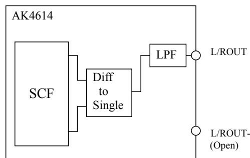
Figure 22. Single-end Output (DOE1-6 bit = “0”)
