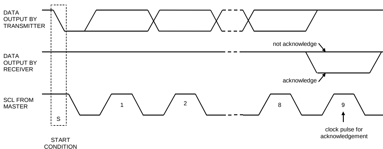
Figure 57. Acknowledge on the I 2 C-Bus
