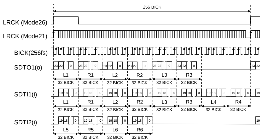
Figure 34. Mode 21/26 Timing (TDM256 Mode)
