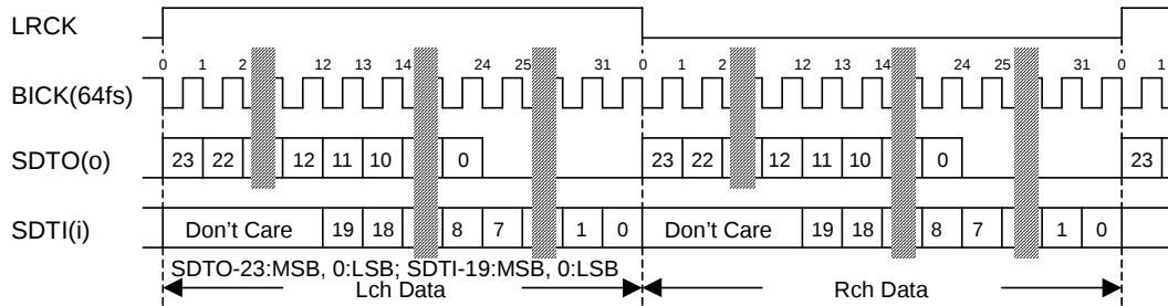
Figure 24. Mode 1/6 Timing (Stereo Mode)
