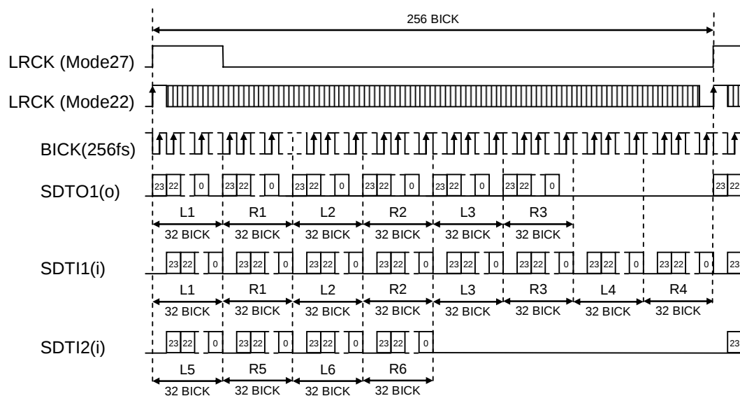
Figure 35. Mode 22/27 Timing (TDM256 Mode)
