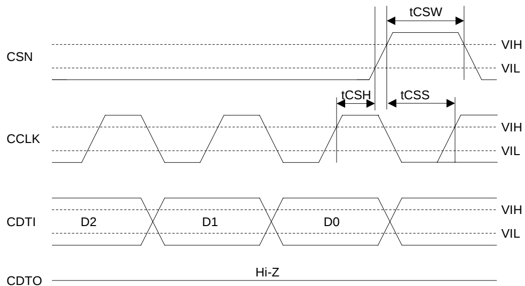
Figure 12. WRITE Data Input Timing (4-wire Serial mode)
