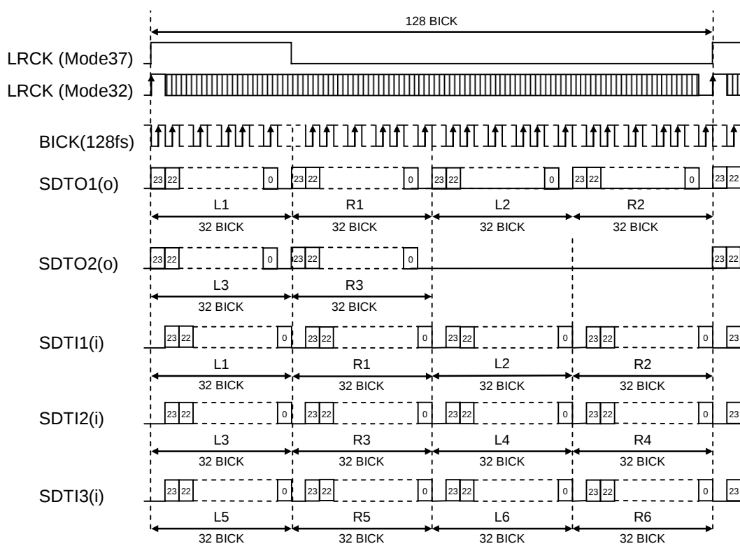
Figure 40. Mode 32/37 Timing (TDM128 Mode)
