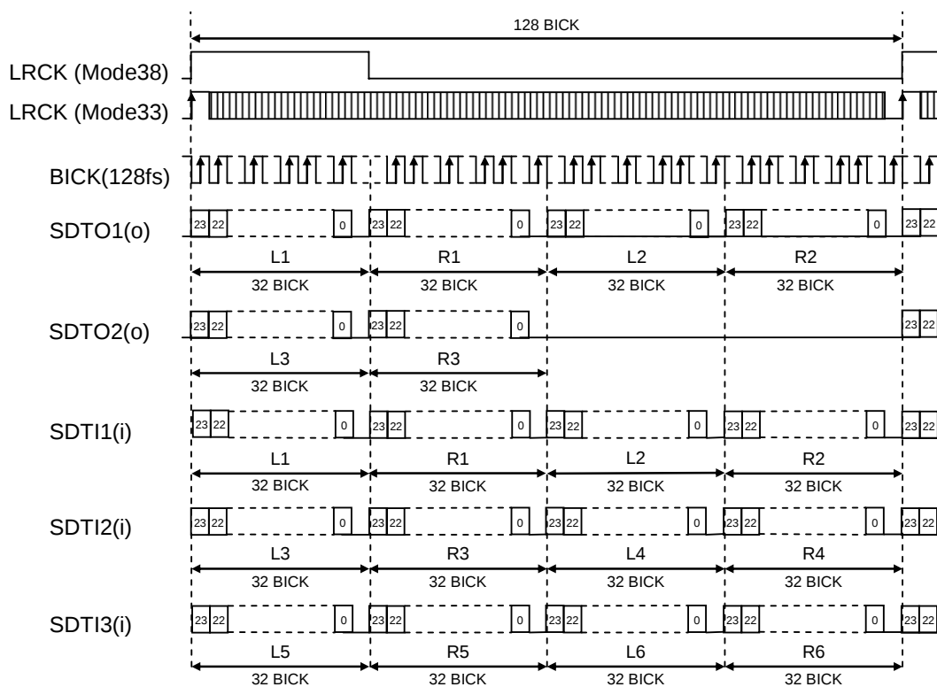
Figure 41. Mode 33/38 Timing (TDM128 Mode)
