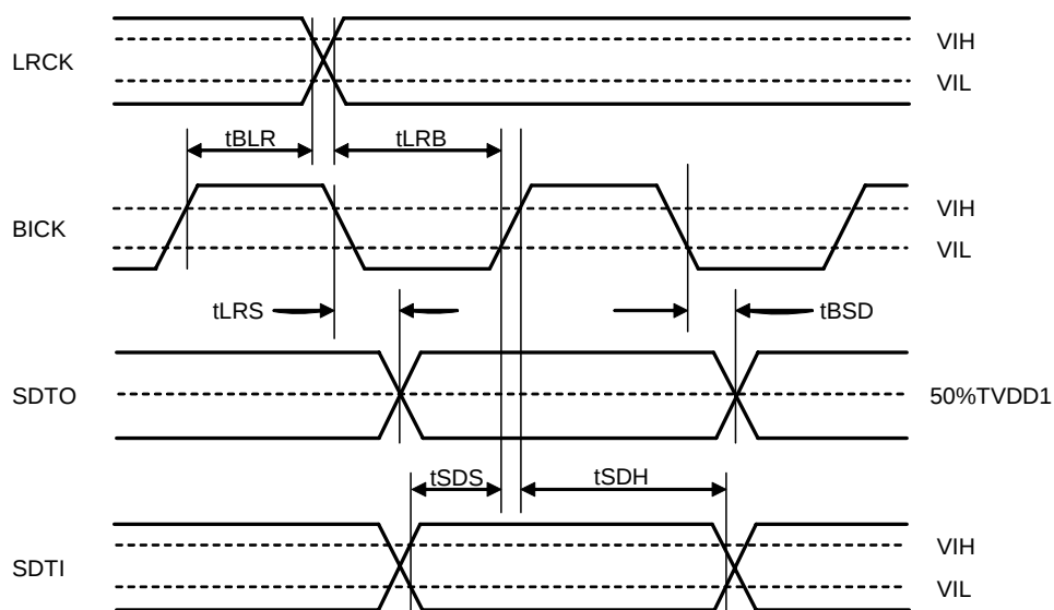
Figure 7. Audio Interface Timing (TDM1/0 bit = "00" & Slave mode)
