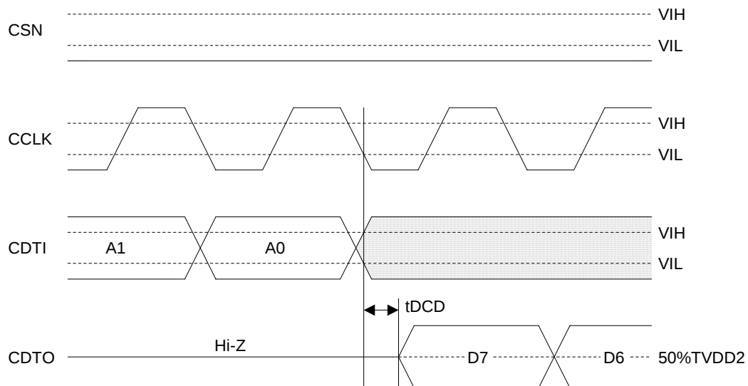
Figure 13. Read Data Output Timing1(4-wire Serial mode)
