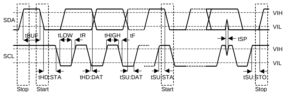
Figure 15. I²C Bus mode Timing
