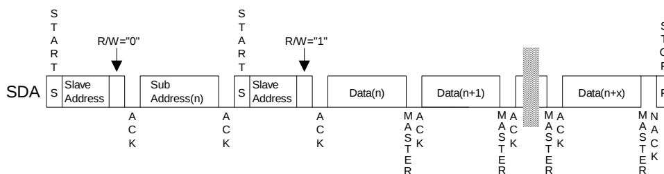
Figure 55. RANDOM ADDRESS READ
