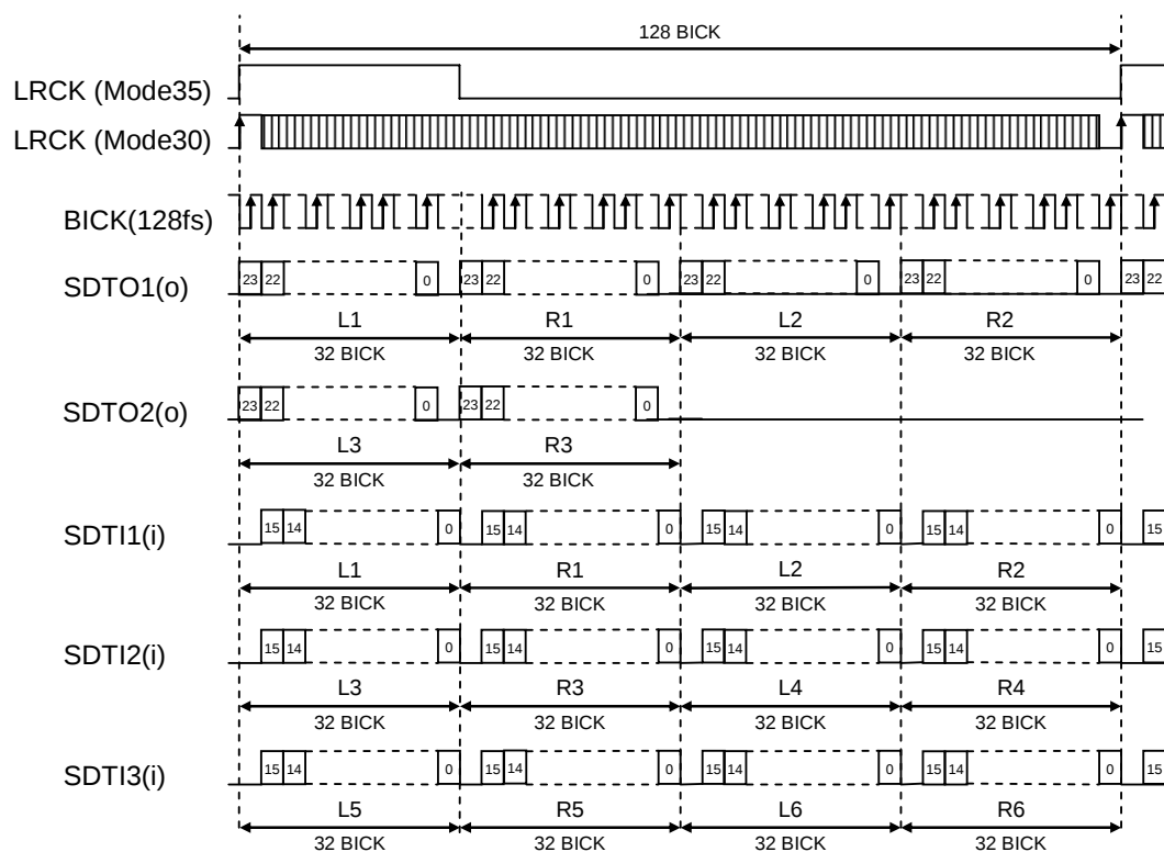
Figure 38. Mode 30/35 Timing (TDM128 Mode)
