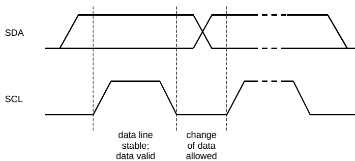
Figure 58. Bit Transfer on the I 2 C-Bus
