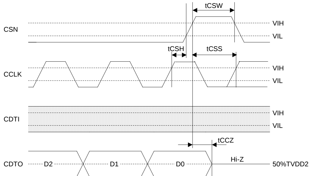
Figure 14. Read Data Output Timing2(4-wire Serial mode)
