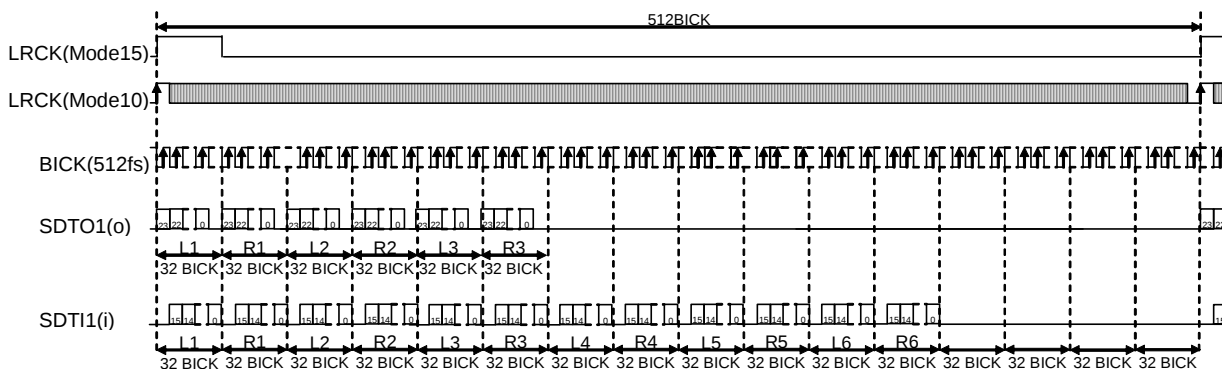
Figure 28. Mode 10/15 Timing (TDM512 Mode)
