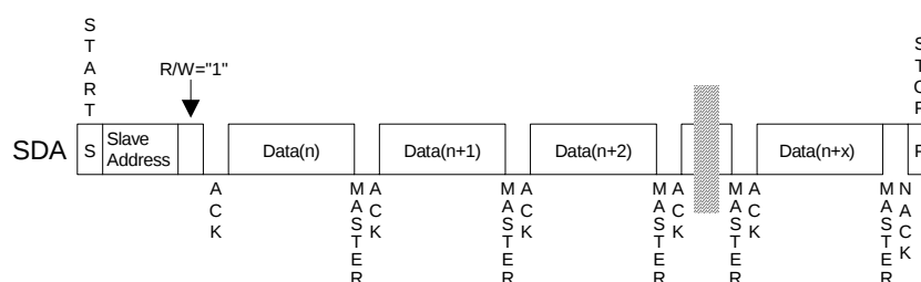
Figure 54. CURRENT ADDRESS READ
