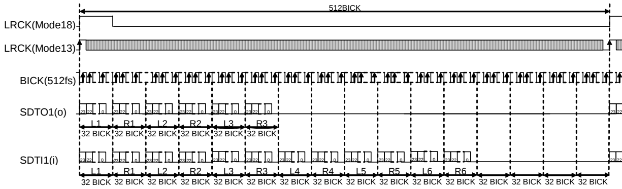
Figure 31. Mode 13/18 Timing (TDM512 Mode)
