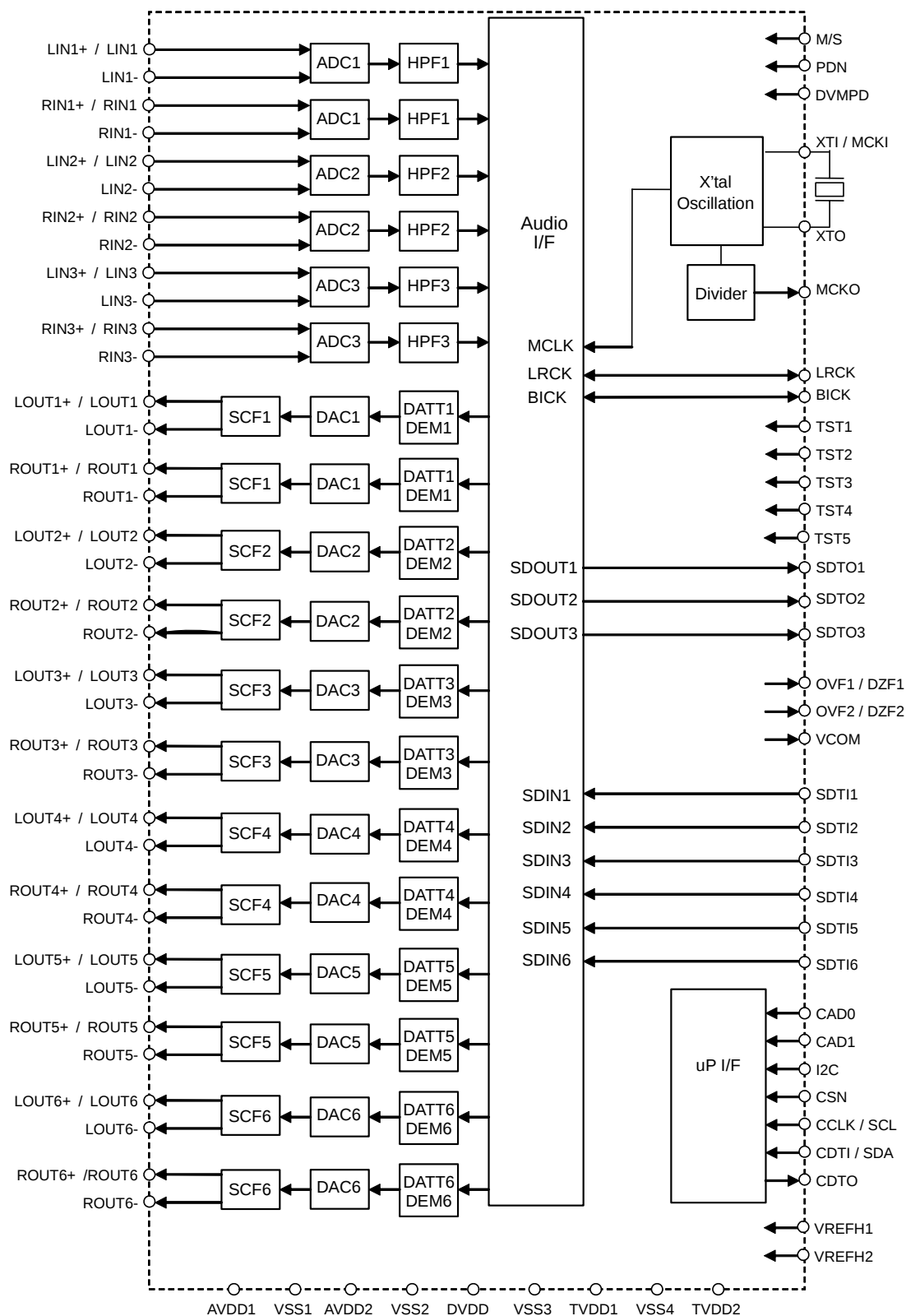
Figure 1. Block Diagram
