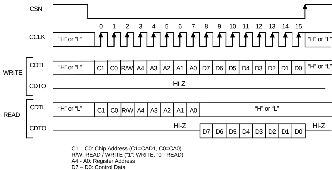
Figure 49. Serial Control I/F Timing
