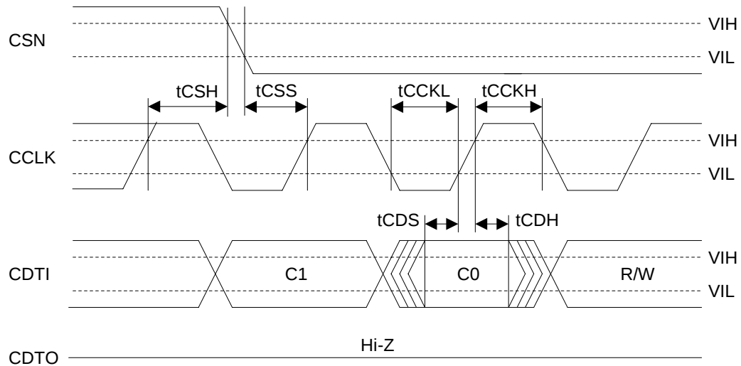
Figure 11. WRITE Command Input Timing (4-wire Serial mode)
