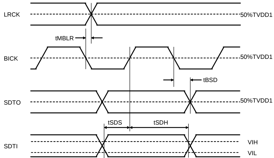
Figure 9. Audio Interface Timing (TDM1/0 bit = "00" & Master mode)
