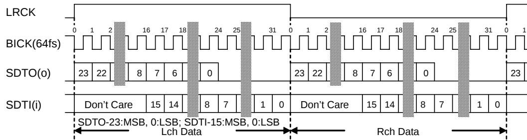
Figure 23. Mode 0/5 Timing (Stereo Mode)
