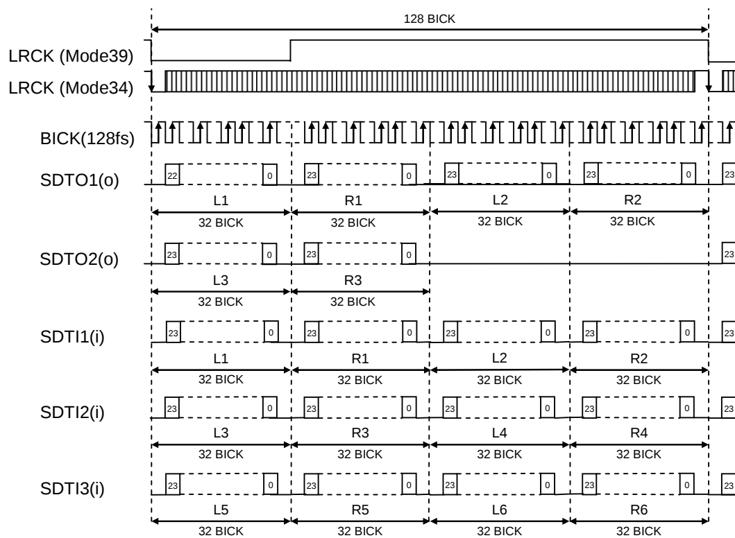
Figure 42. Mode 34/39 Timing (TDM128 Mode)
