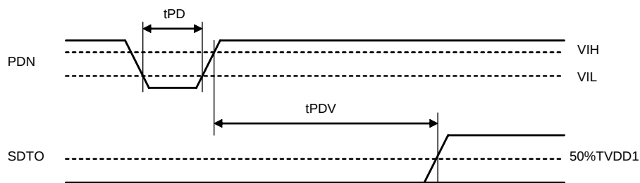
Figure 16. Power-down &amp; Reset Timing
