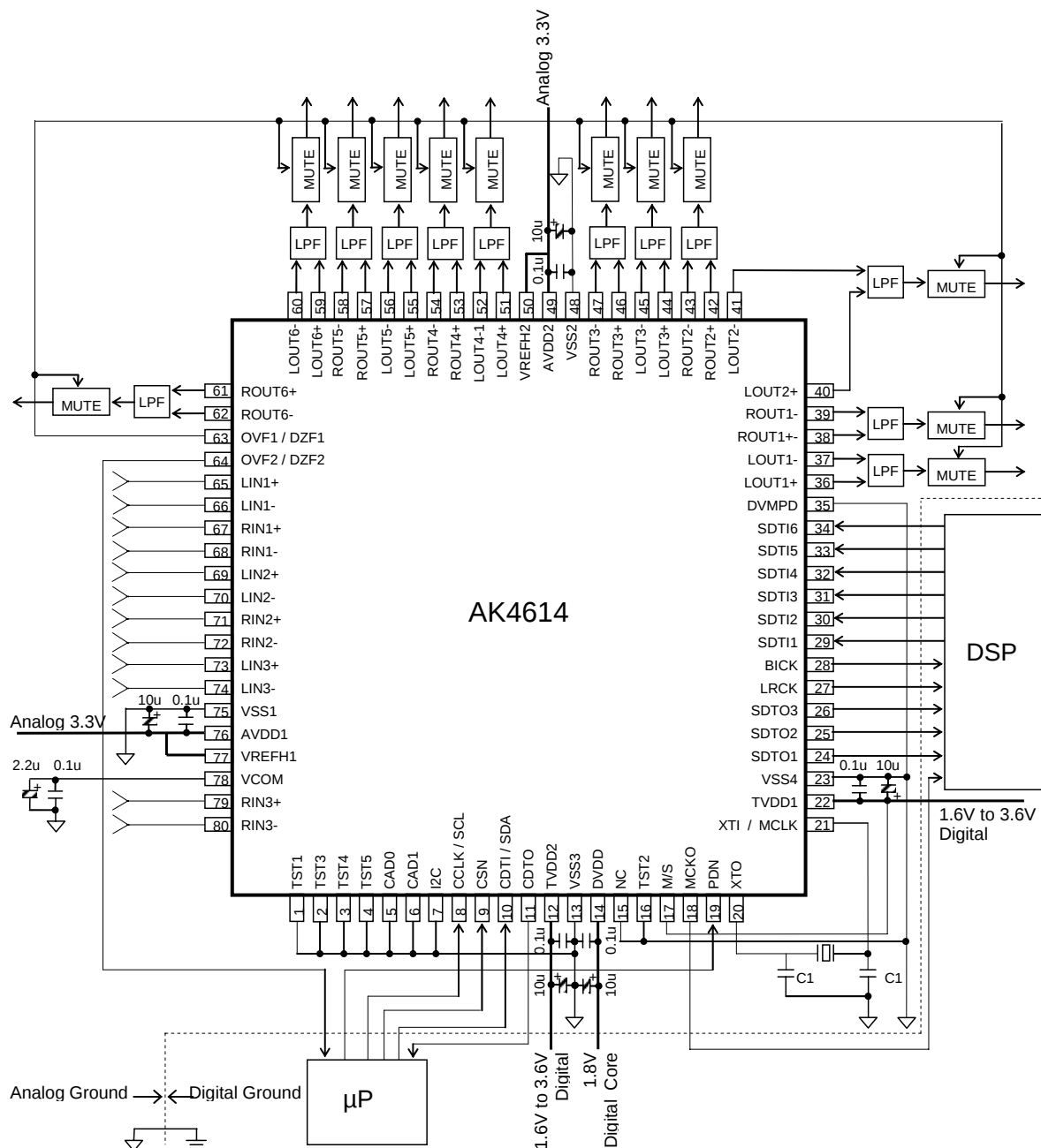
Figure 59. Typical Connection Diagram1
