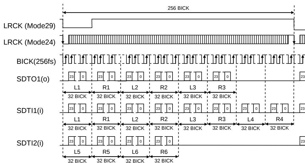
Figure 37. Mode 24/29 Timing (TDM256 Mode)
