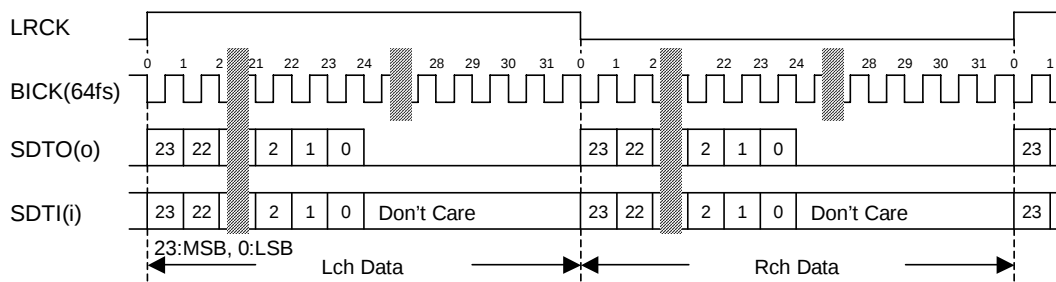
Figure 26. Mode 3/8 Timing (Stereo Mode)
