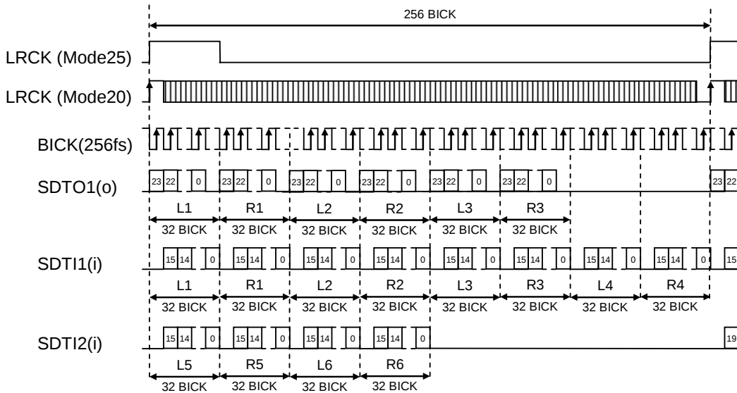
Figure 33. Mode 20/25 Timing (TDM256 Mode)
