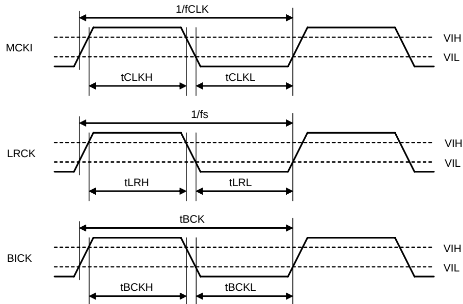
Figure 4. Clock Timing (Except TDM1/0 bit = "00" & Slave mode)
