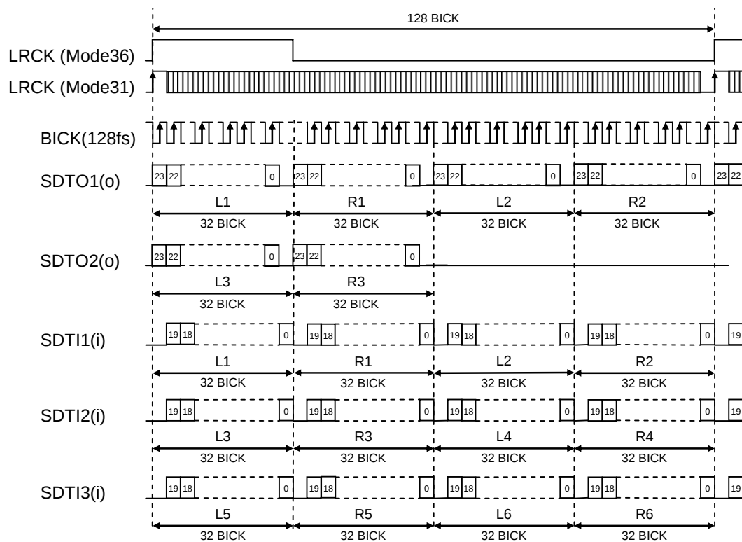
Figure 39. Mode 31/36 Timing (TDM128 Mode)
