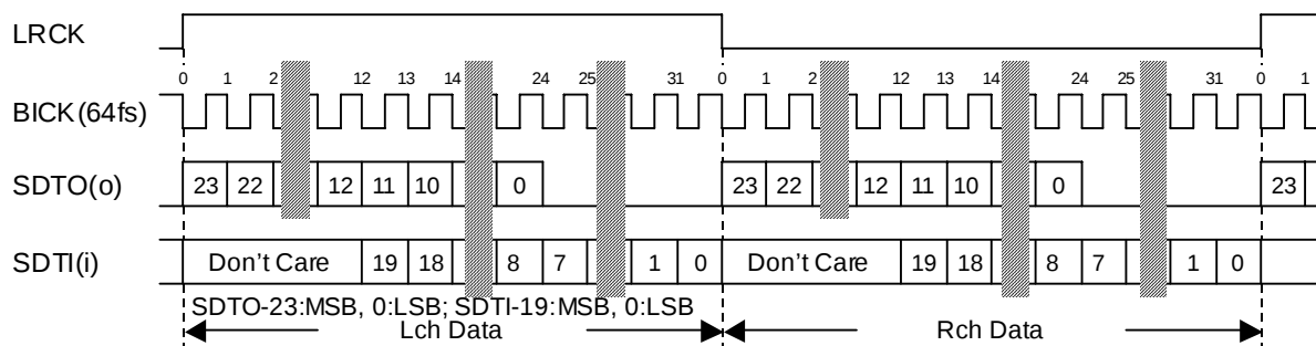
Figure 1. Mode 0, 4 Timing
