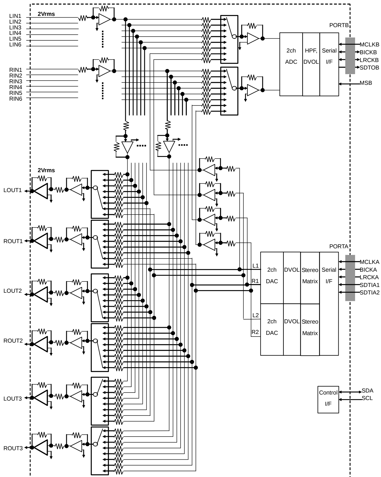
AK4682 Block Diagram
