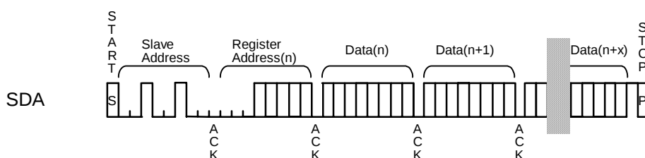
Figure 20. WRITE Operation
