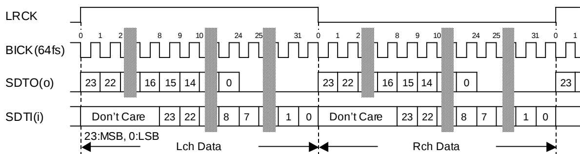
Figure 2. Mode 1, 5 Timing
