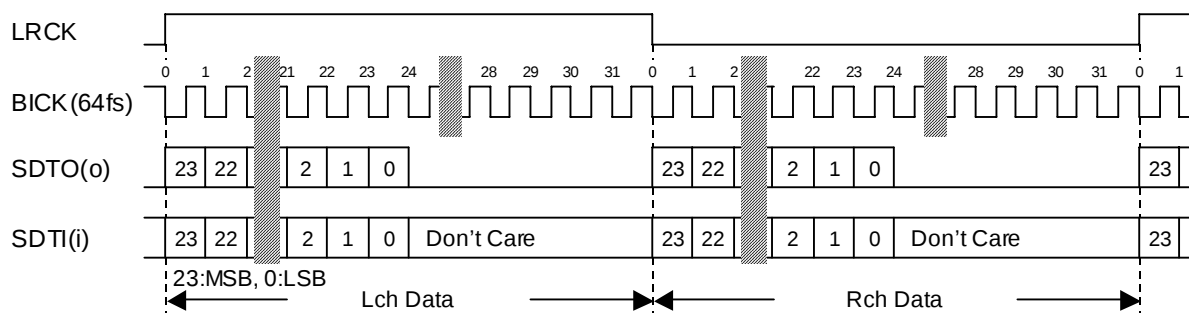
Figure 3. Mode 2, 6 Timing
