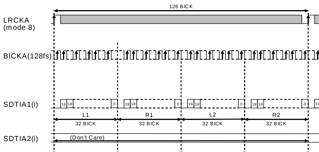
Figure 5. Mode 8 Timing
