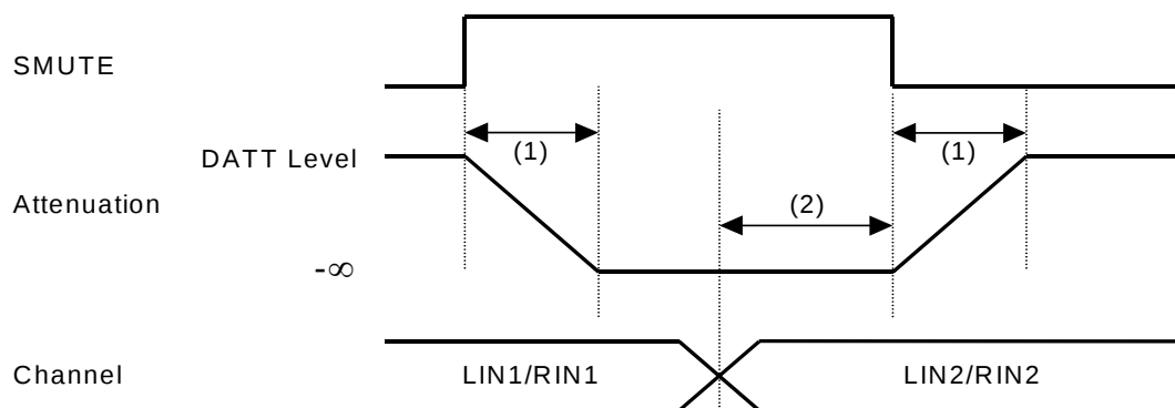
Figure 11. Input channel switching sequence example
