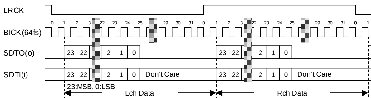
Figure 4. Mode 3, 7 Timing
