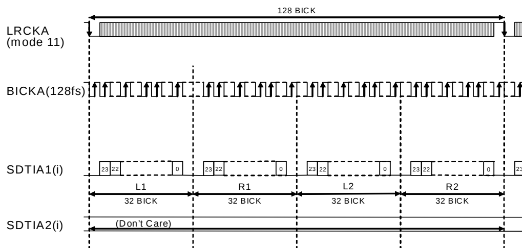
Figure 8. Mode 11 Timing
