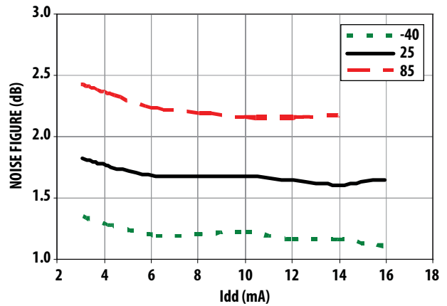
Figure 8. NF vs. Idd at Vdd = 2.7V
