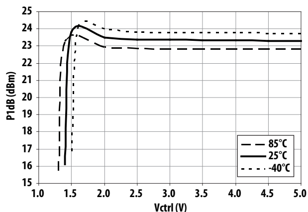
Figure 31. P1dB vs Control Voltage and Temperature at 900MHz
