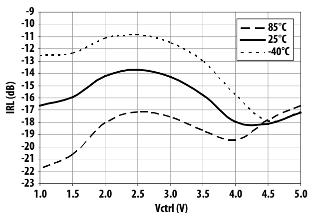
Figure 33. IRL vs Control Voltage and Temperature at 900MHz
