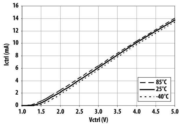
Figure 51. Current ( I_{ctrl} ) vs Control Voltage and Temperature
