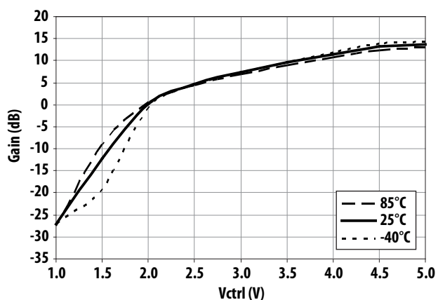
Figure 32. Gain vs Control Voltage and Temperature at 900MHz
