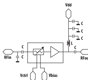
Figure 1. Simplified Schematic diagram
