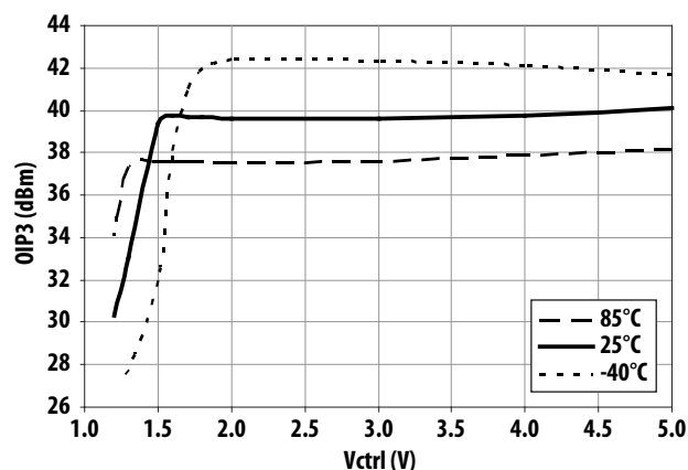
Figure 30. OIP3 vs Control Voltage and Temperature at 900MHz
