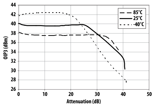
Figure 36. OIP3 vs Attenuation and Temperature at 900MHz
