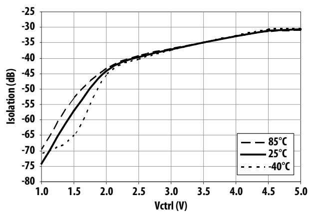
Figure 35. Isolation vs Control Voltage and Temperature at 900MHz
