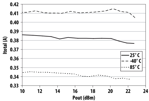
Figure 58. Idd_total vs Pout (Dual Carrier Signal) at 2140 MHz
