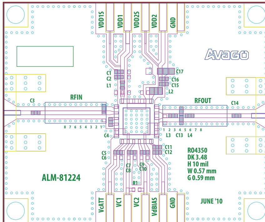
Figure 72. Demo board diagram of application circuit for 2140 MHz
