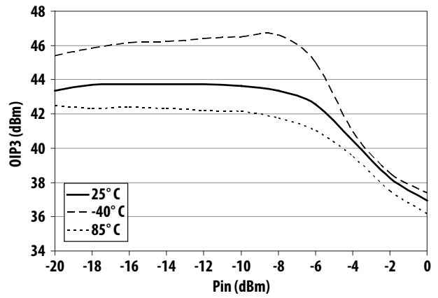
Figure 15. OIP3 vs Pin at 1485 MHz
