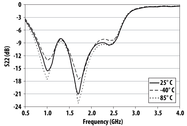
Figure 33. S22 vs Freq at 1960 MHz
