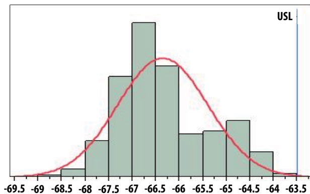
Figure 4. ACLR (Dual-Carrier Signal) at 12 dBm output power; Nominal = -66.6 dBc, USL = -63.5 dBc
