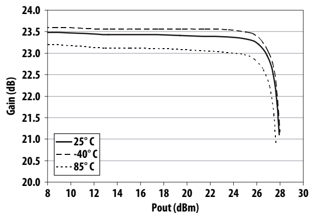
Figure 53. Gain vs Pout at 2140 MHz
