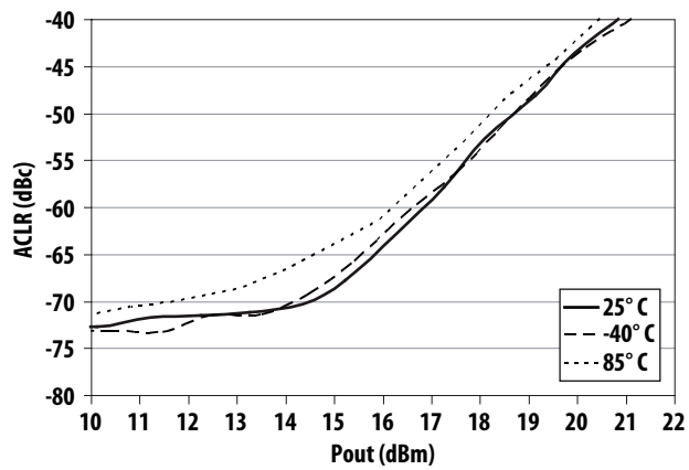
Figure 56. ACLR (Single Carrier Signal) vs Pout at 2140 MHz
