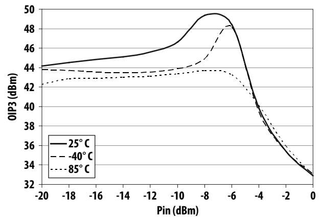
Figure 27. OIP3 vs Pin at 1840 MHz
