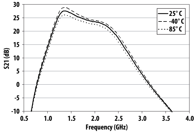
Figure 10. S21 vs Freq at 1485 MHz
