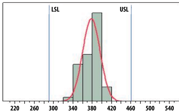
Figure 1. I_{dd\_total} at V_{dd} = 5\text{ V} ; LSL = 290 mA, Nominal = 383 mA, USL = 460 mA
