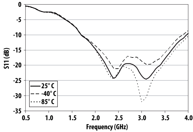
Figure 44. S11 vs Freq at 2140 MHz
