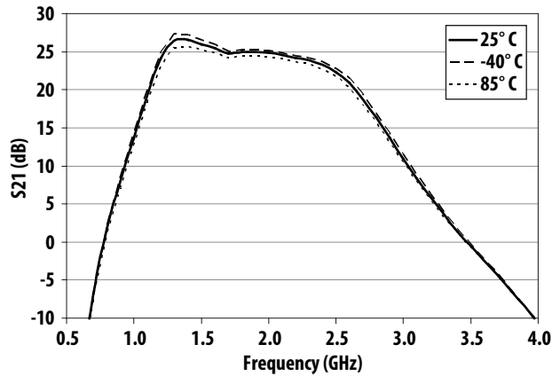
Figure 22. S21 vs Freq at 1840 MHz
