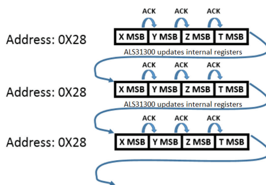
Figure 7: Fast Loop Mode
