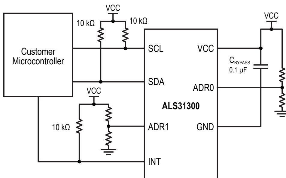
Figure 2: Typical Application
