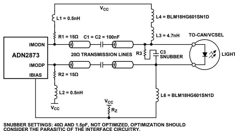
Figure 36. Recommended Differential Drive Circuit
