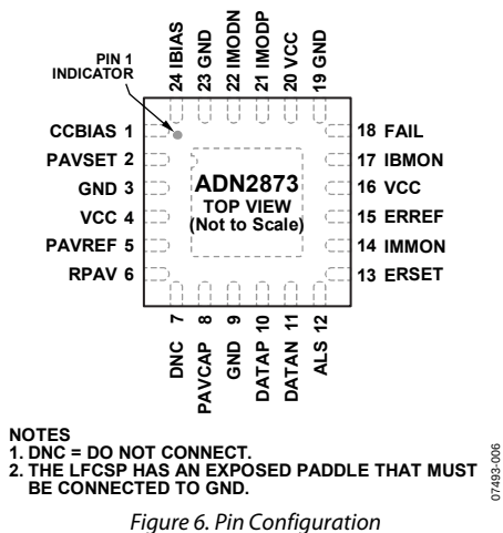
Figure 6. Pin Configuration
