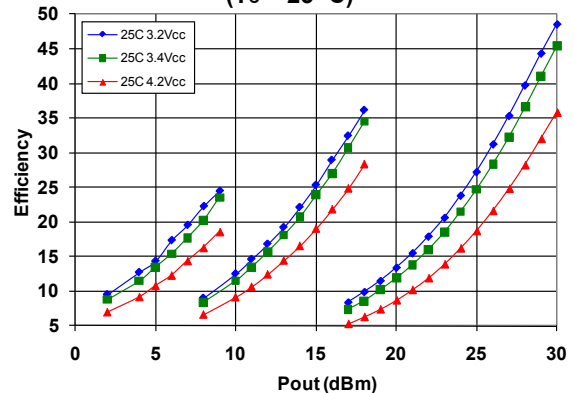
Figure 6: LTE PAE (%) over Voltage ( T_c = 25 °C)
