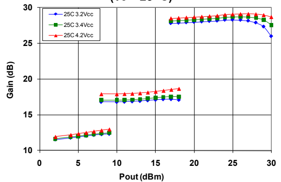
Figure 4: LTE Gain (dB) over Voltage ( T_c = 25 °C)
