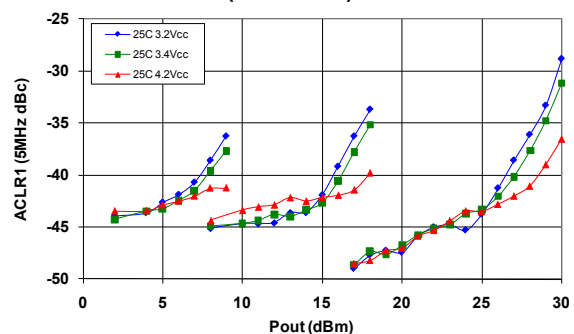
Figure 8: LTE ACLR1 (dBc) over Voltage ( T_c = 25 °C)
