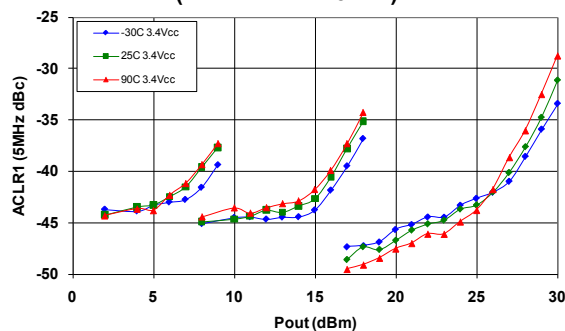
Figure 7: LTE ACLR1 (dBc) over Temperature ( V_{BATT} = V_{CC} = 3.4 V)
