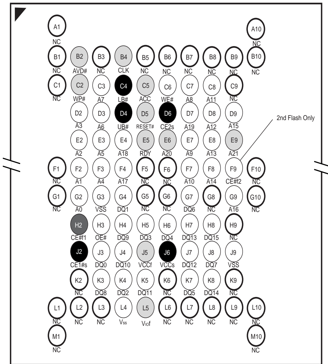
93-Ball FBGA Top View
