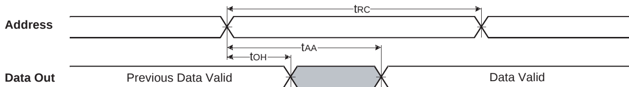
Figure 26. Timing Waveform of Read Cycle 1
