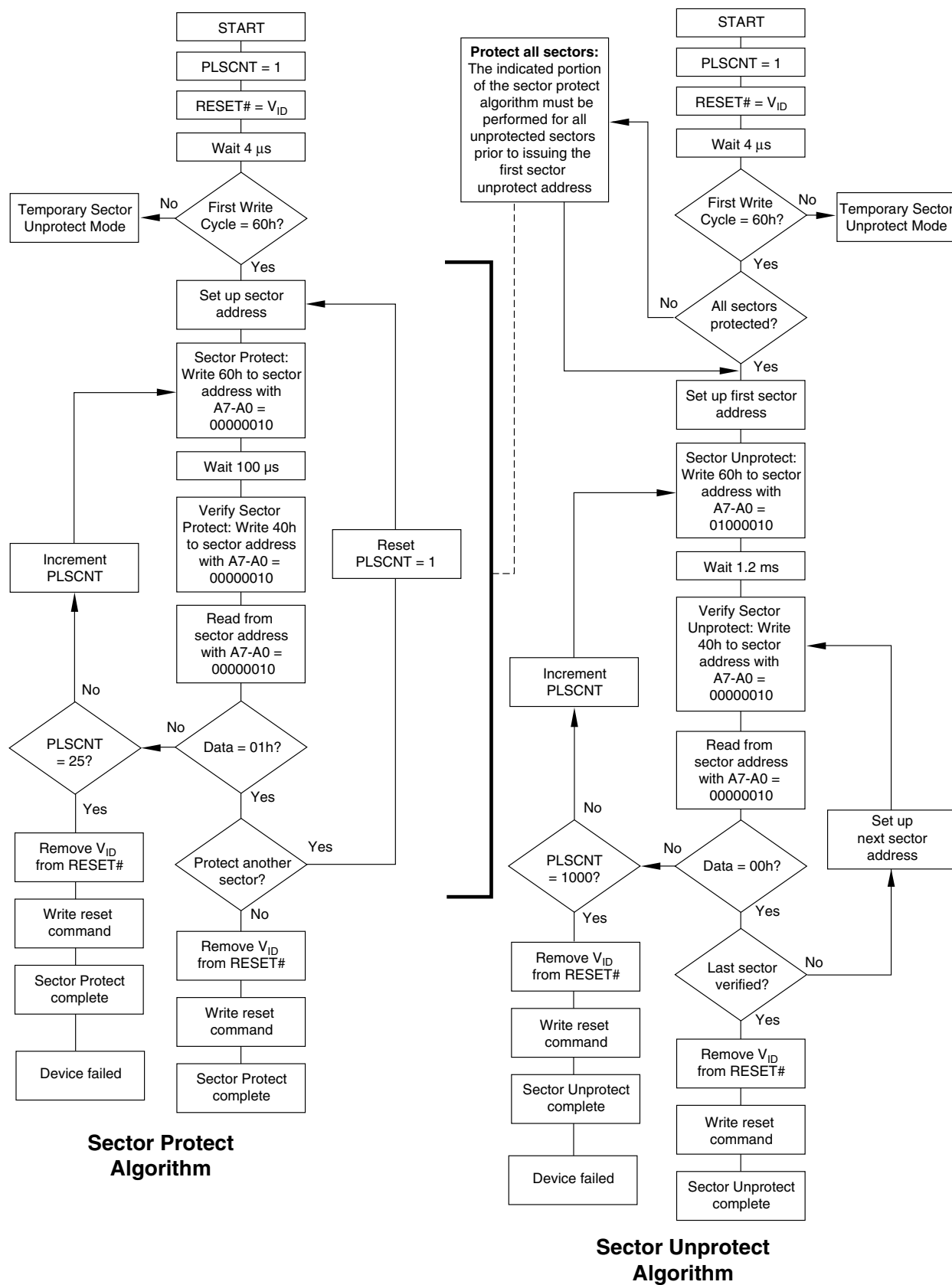
Figure 1. In-System Sector Protection/ Sector Unprotection Algorithms
