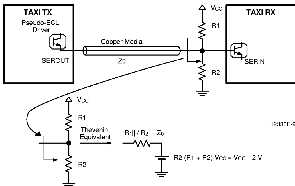
Figure 5-2 Parallel Termination
