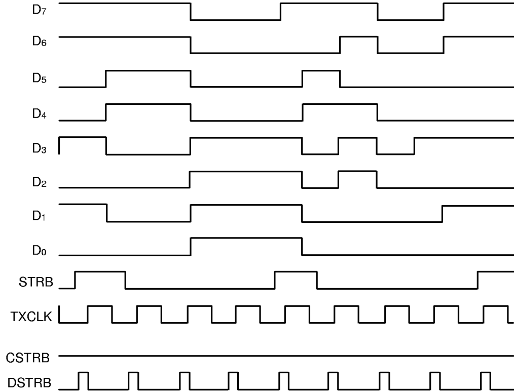
Figure 17 AUTORUN ACK 0 (No Sync Between Data Bytes)
