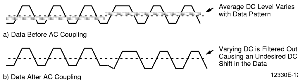
Figure 5-5 Baseline Wander
