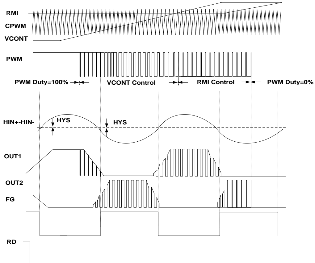
Truth Table for Various Modes with VCONT/RMI PIN
