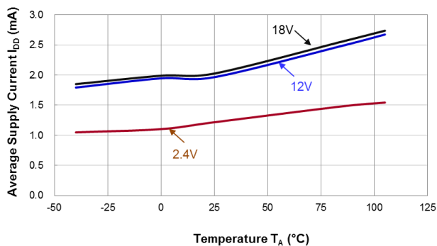
Average Supply Current vs. Temperature
