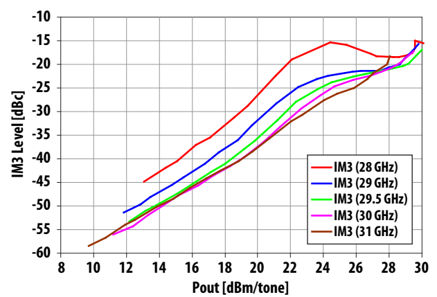
Figure 6. IM3 level (dBc) vs. Output power/ton
