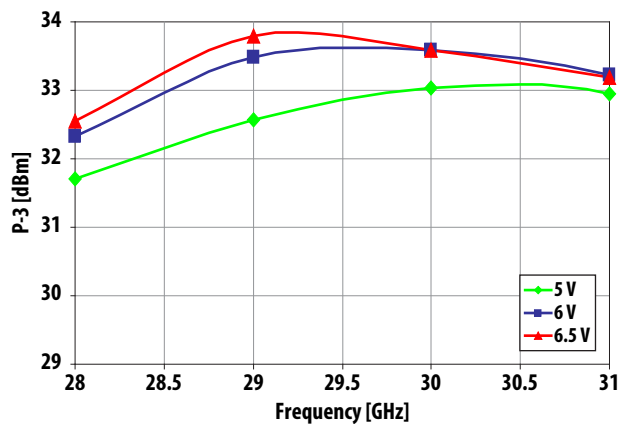
Figure 17. P_{3\text{dB}} (dBm) Frequency Sweep
