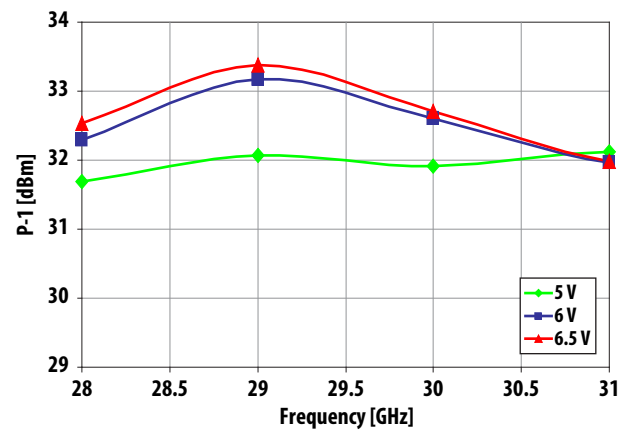
Figure 16. P_{1\text{dB}} (dBm) Frequency Sweep
