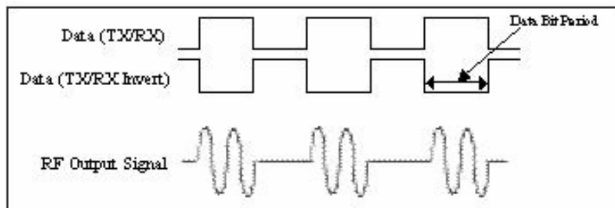
Figure 8: Transmit Waveforms
