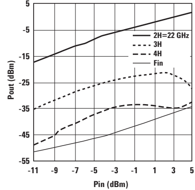
Figure 4. Typical Output Power against Fundamental 3 rd and 4 th Harmonic suppression vs. P_{in} ( 2H = 22\text{ GHz} ).
