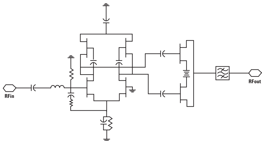
Figure 10. AMMC-6140 simplified schematic.
